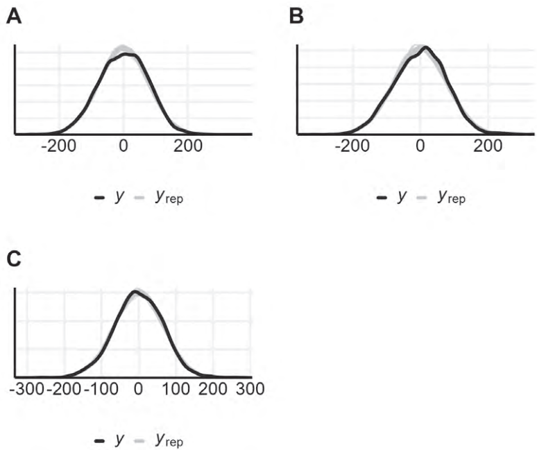
Figure 2 – Predictive posterior distribution of 50 simulated datasets based on the model (in grey) with the distribution of the original data plotted on top (in black) for (A) Experiment 1, (B) Experiment 2, and (C) Experiment 3.
