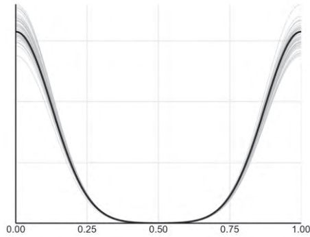
Figure 5 – Predictive posterior distribution of 50 simulated datasets based on the model (in grey) with the distribution of the original data plotted on top (in black) for the preference test model.
