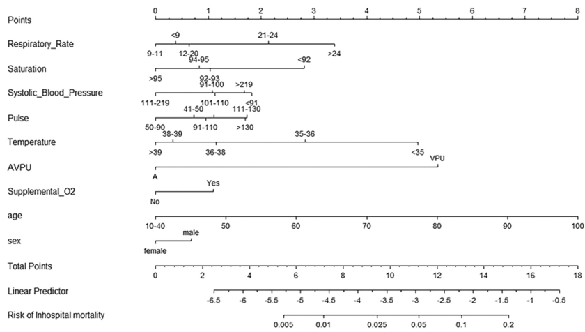
Nomogram for a recalibrated National Early Warning Score +age+sex
