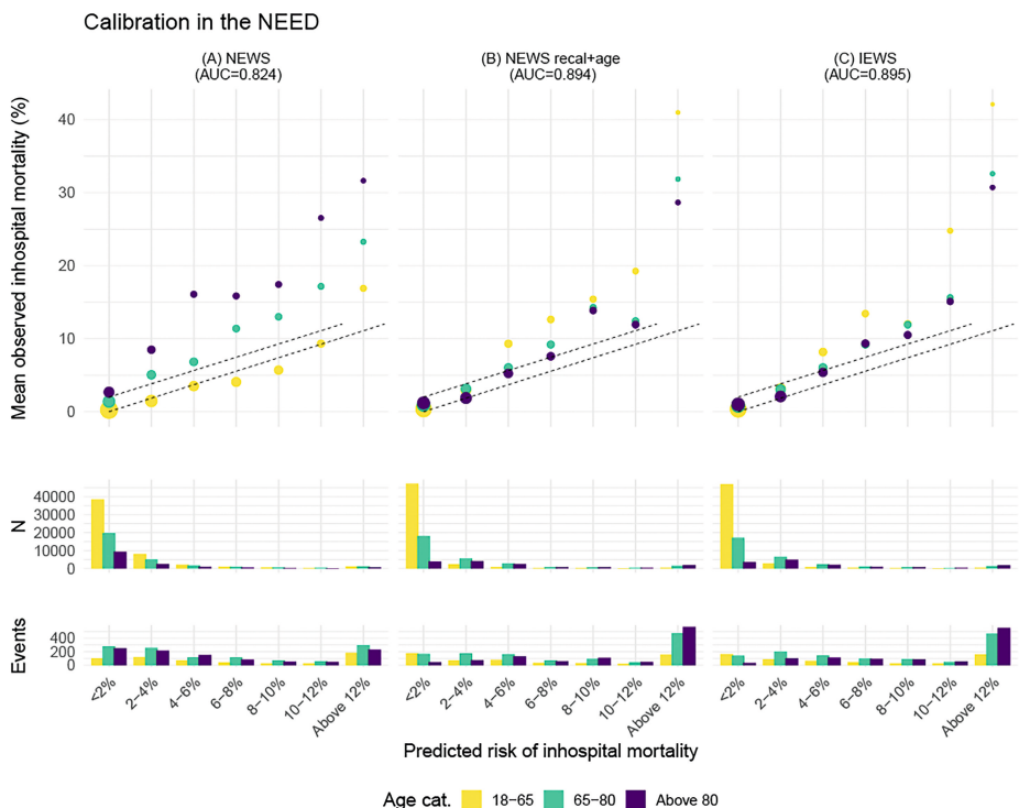
Figure 1 Internal calibration plots for the NEED (Netherlands Emergency department Evaluation Database) for (A) the National Early Warning Score (NEWS), (B) a recalibrated NEWS + age and (C) a recalibrated NEWS+age+sex (the International Early Warning Score (IEWS)). The predicted in-hospital mortality was categorized in steps of 2% in the relevant risk range. Calibration was assessed in three different age categories (18-65y, 66-80y,>80y). The dotted lines represent ideal calibration. The size of the dots indicates the precision of the estimate for observed inhospital mortality in each risk group, the larger, the higher the precision based on the inverse of the standard deviation. Below the calibration figures are the distribution of patients and outcomes presented for all three scores in histograms.
