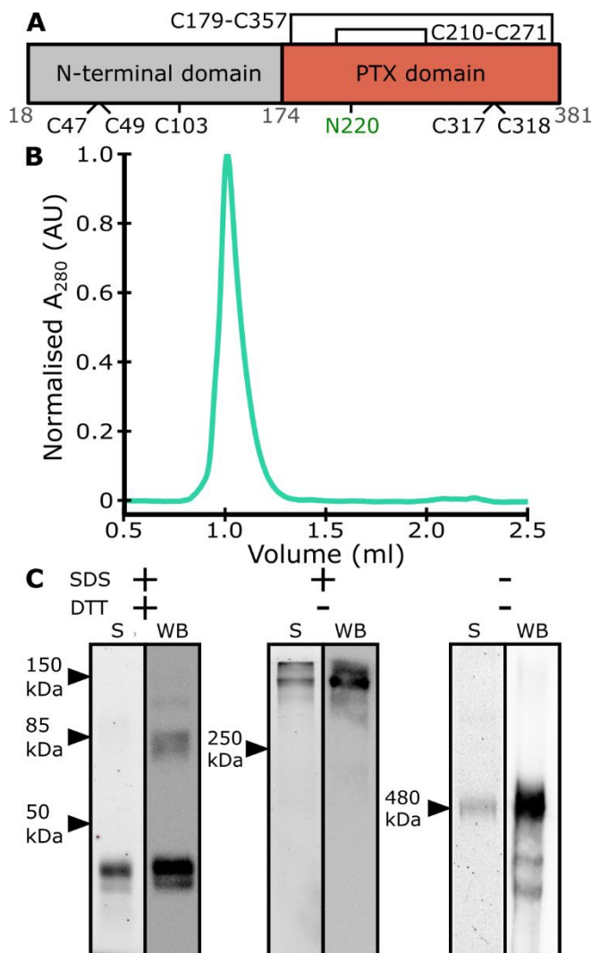
Figure 1. Purification of recombinant human PTX3. (A) Schematic of the PTX3 monomer, indicating sites of glycosylation (N220) and disulfide bonds. Intra-monomeric disulfide bonds are shown as closed loops. Numbering of residues is shown in grey. (B) SEC elution profile of PTX3 after Ni-NTA affinity and SEC purification. (C) Gel electrophoretic profiles based on TCE staining (S) and Western blots (WB) of PTX3 after purification under in the presence of SDS and/or DTT. Arrows indicate standard protein markers of the indicated molecular weight.
