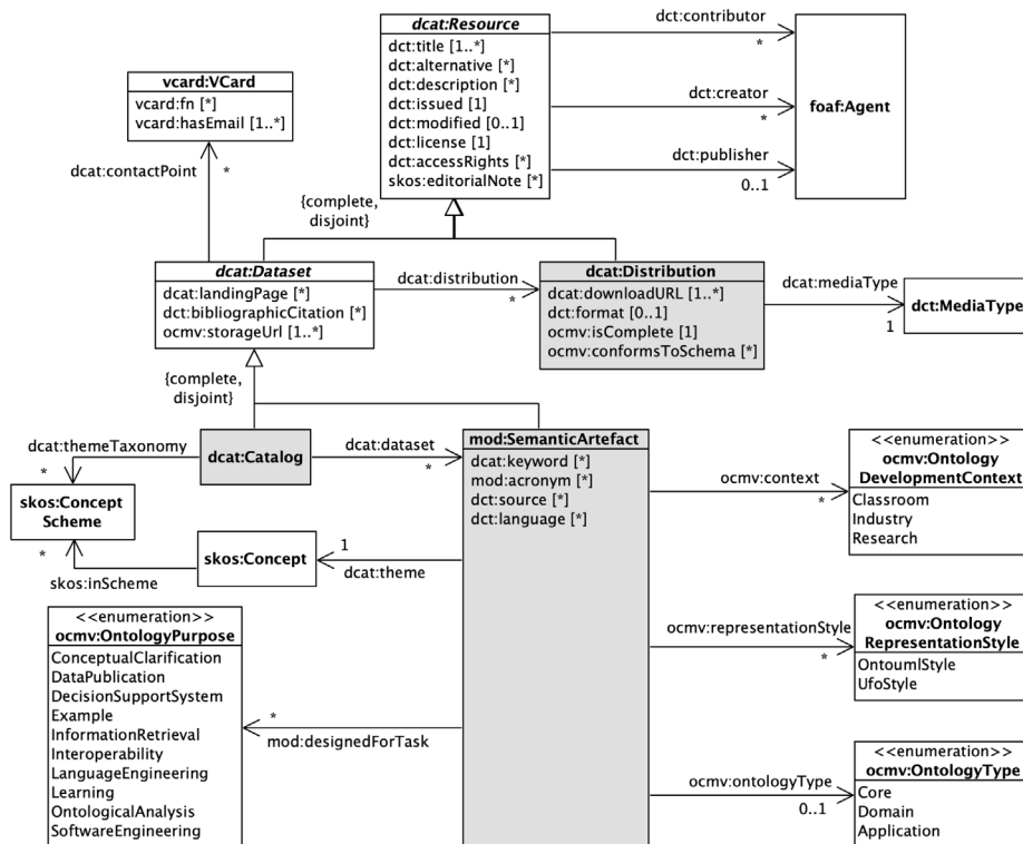
Fig. 9. The metadata schema for the OntoUML/UFO Catalog ( dcatalog:Catalog ), the conceptual models ( mod:SemanticArtefact ), and their distributions ( dcatalog:Distribution ) described as a UML class diagram.
