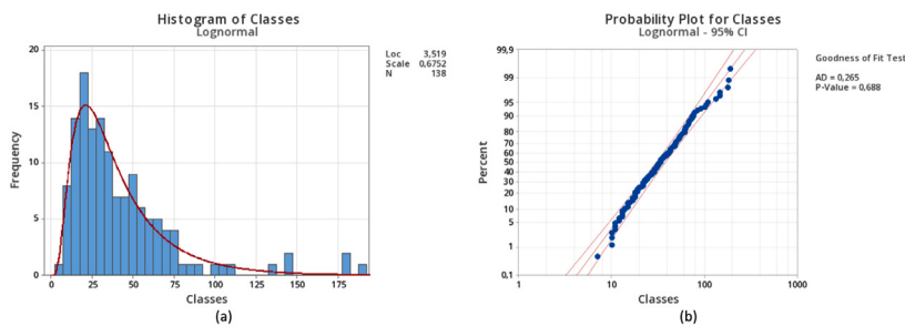
Fig. 12. (a) Histogram of classes and (b) probability plot for classes.
