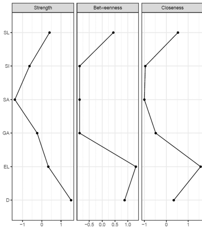
Fig. 2. Centrality indices of the network. X-axis represents the standardized z-scores of the edge strength, betweenness, and closeness. Y-axis represents the nodes (variables). SL = Social Loneliness, SI = Social Isolation, SA = Social Anxiety, GA = General Anxiety, EL = Emotional Loneliness, D = Depression.
