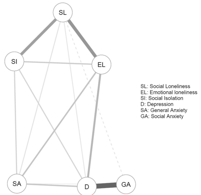
Fig. 1. Estimated network between social loneliness, emotional loneliness, social isolation, social anxiety, depression, and general anxiety. Solid lines indicate positive associations while dashed lines indicate negative ones. The thickness and brightness of the edges represent the strength of the relationships. As a reference, the weight of the edge between EL and SL is 0.43. The location of the nodes in the network represents its frequency of connecting and closeness to other variables in the network.
