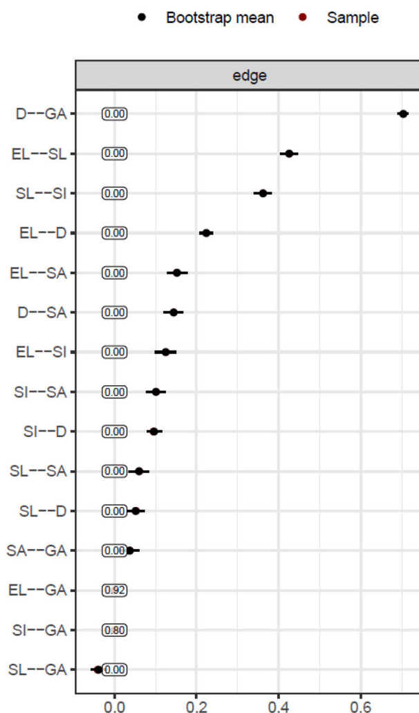
Fig. 2. Bootstrapped coefficient intervals (CIs) showing the proportion (%) of time an edge between two nodes was estimated as being 0.
