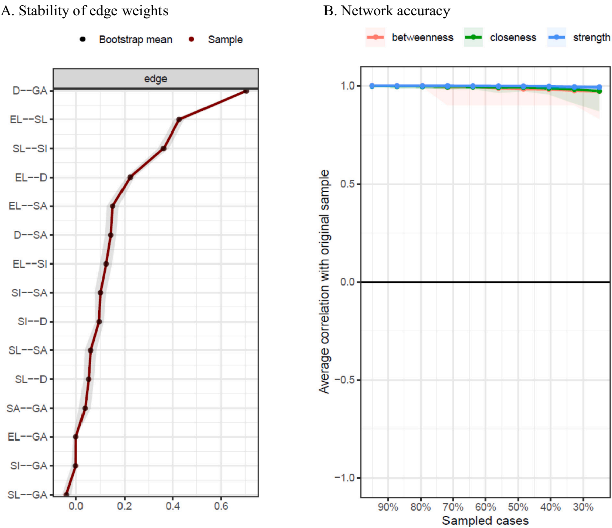
Fig. 1. A: Non-parametric bootstrapping results to assess edge weights stability of the network. X-axis shows the strength of the edges and the Y-axis represent the 95 % bootstrapped coefficient intervals (CIs) of pair-wise edges. B: Case bootstrapping results to assess network accuracy. X-axis represents the percentage of sampled cases and the Y-axis shows the average correlation with the original sample.
