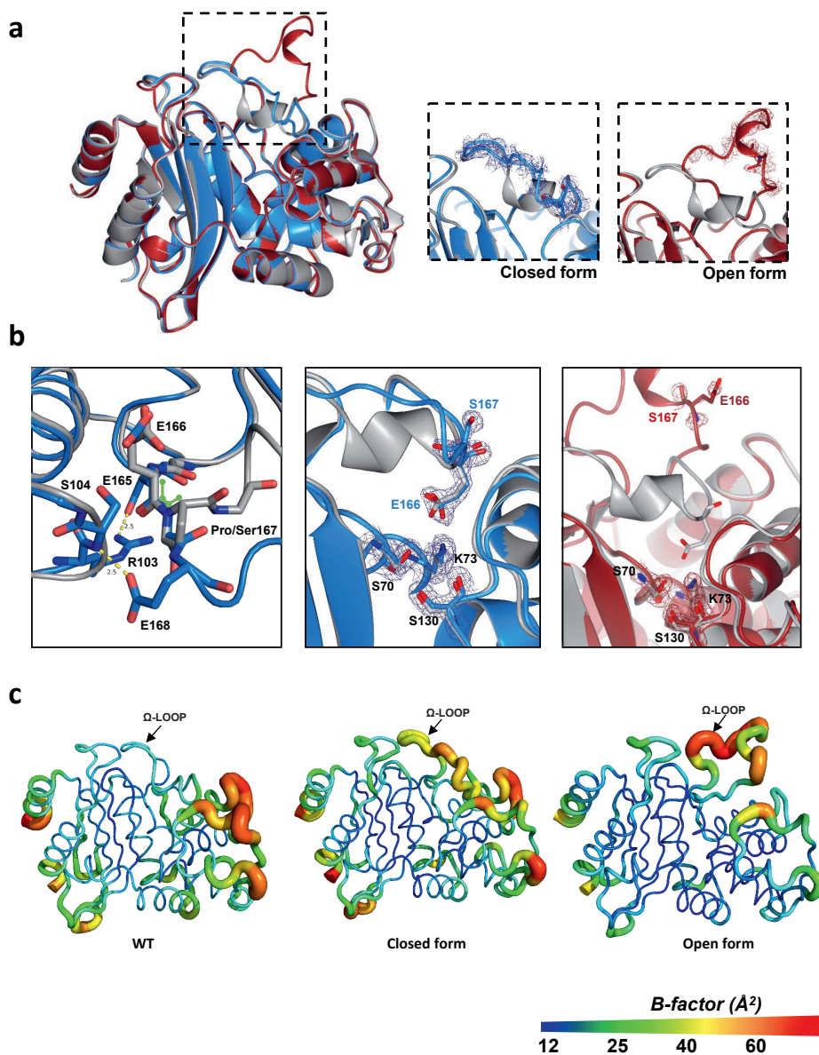
Figure 2.5 Crystal structure of the open and closed forms of BlaC P167S. a) X-ray crystal structure of the resting state of BlaC P167S. The open form is shown in red, and the closed form in blue; both forms are shown overlaid with the WT BlaC structure (grey, PDB 2GDN 72 ) for reference. The images on the right show a close-up of the \Omega -loop. The residue shown in sticks is Ser167; b) The positions of Arg103, Ser104, Ser167, Glu165, Glu168, Glu166,
