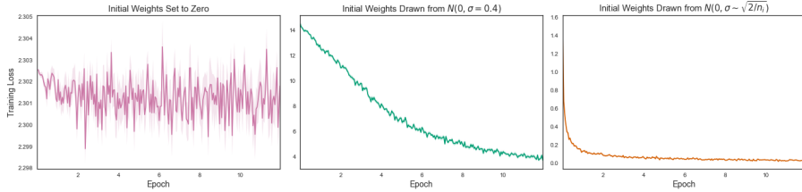
Figure 3.9: Comparative visualization of training loss trajectories using different weight initialization strategies for a CNN on the MNIST dataset. Each subplot displays the 10-batch rolling average of the loss incurred during the training of a basic CNN on the MNIST dataset, which consists of 60000 images of handwritten digits. The network was trained for a total of 12 epochs with a batch size of 128 images for each weight initialization strategy. The left plot shows the model with weights initialized to zero, exhibiting high variability and poor convergence. The middle plot illustrates weights initialized from a normal distribution with a standard deviation of 0.4, showing better, yet suboptimal performance. The right plot demonstrates the superior performance of weights initialized from a normal distribution with variance scaled inversely with the number of neuron inputs, yielding the most stable convergence and significantly lower loss. This strategy led to a network achieving over 99% validation accuracy and a notably smaller final loss compared to the other two methods, underscoring the importance of proper weight initialization in neural network training.(source: [65]).
