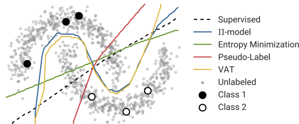
Figure 3.18: In the “two-moons” dataset, virtual adversarial training (VAT) and temporal ensembling (pi-model) methods were able to learn a highly accurate decision boundary with a relatively small amount of labeled data, specifically 6 data points depicted as large white and black circles in this figure. In contrast, Pseudo-Labeling was found to be inadequate in this context, resulting in the learning of a linear decision boundary. This highlights the limitations of Pseudo-Labeling as compared to VAT and pi-model in this specific dataset (source: [121]).
