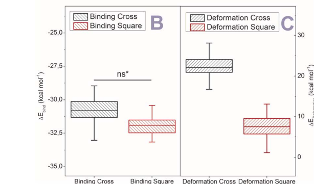
Fig. 9 (A) GFN2-xTB Hamiltonian and analytical linearized Poisson-Boltzmann (ALPB) optimized model structures of two possible environments around copper (square and cross representing 1 and 2 respectively) (Pd = yellow; Cu = green (tetrahedral orientation of ligands)). (B) Binding energies for the square and cross fragments displayed in (A). (C) Deformation energies for the construction of 1 or 2 (Fig. 8A) with the copper located in the squares and in crosses respectively.
