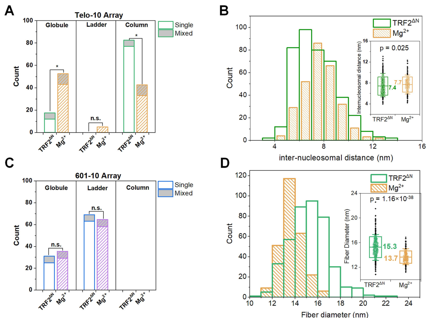
Figure 3. Characterisation of telomeric and 601 array compaction.
