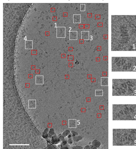
F Telo-4 array + TRF2 dimer (0.5 dimer/157 bp of DNA)
