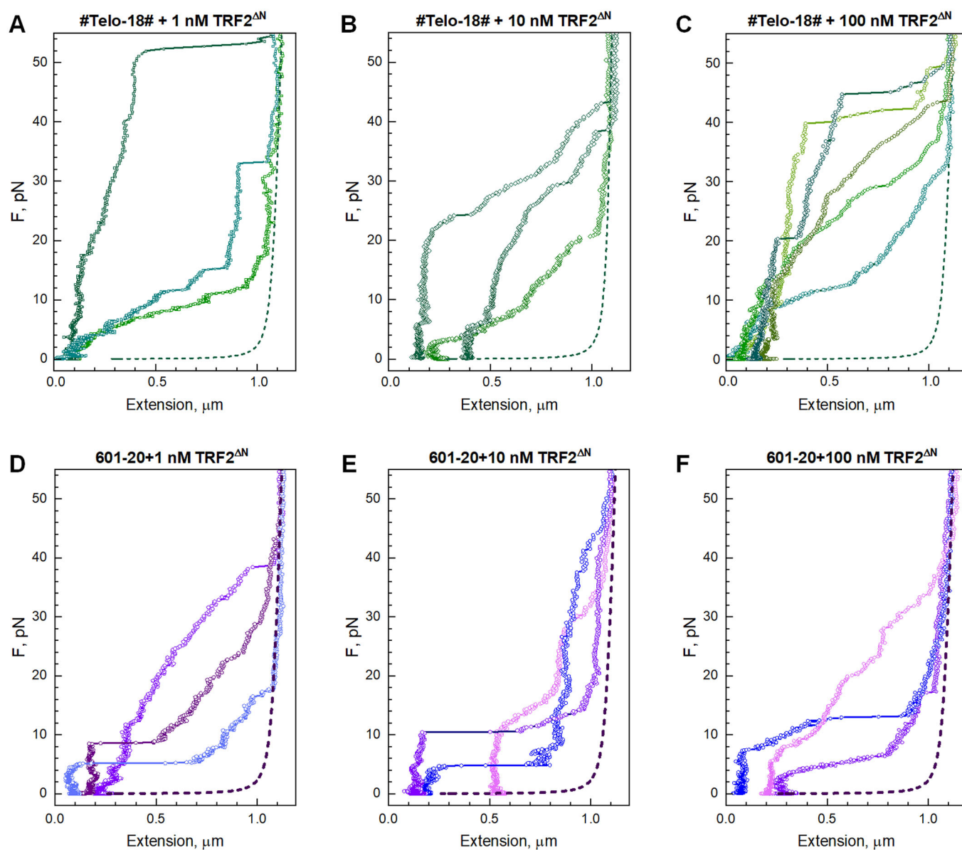
Figure EV4. Examples of stretching curves of the #Telo-18# and 601-20 arrays which cannot be reliably fitted by the current statistical mechanics model.
