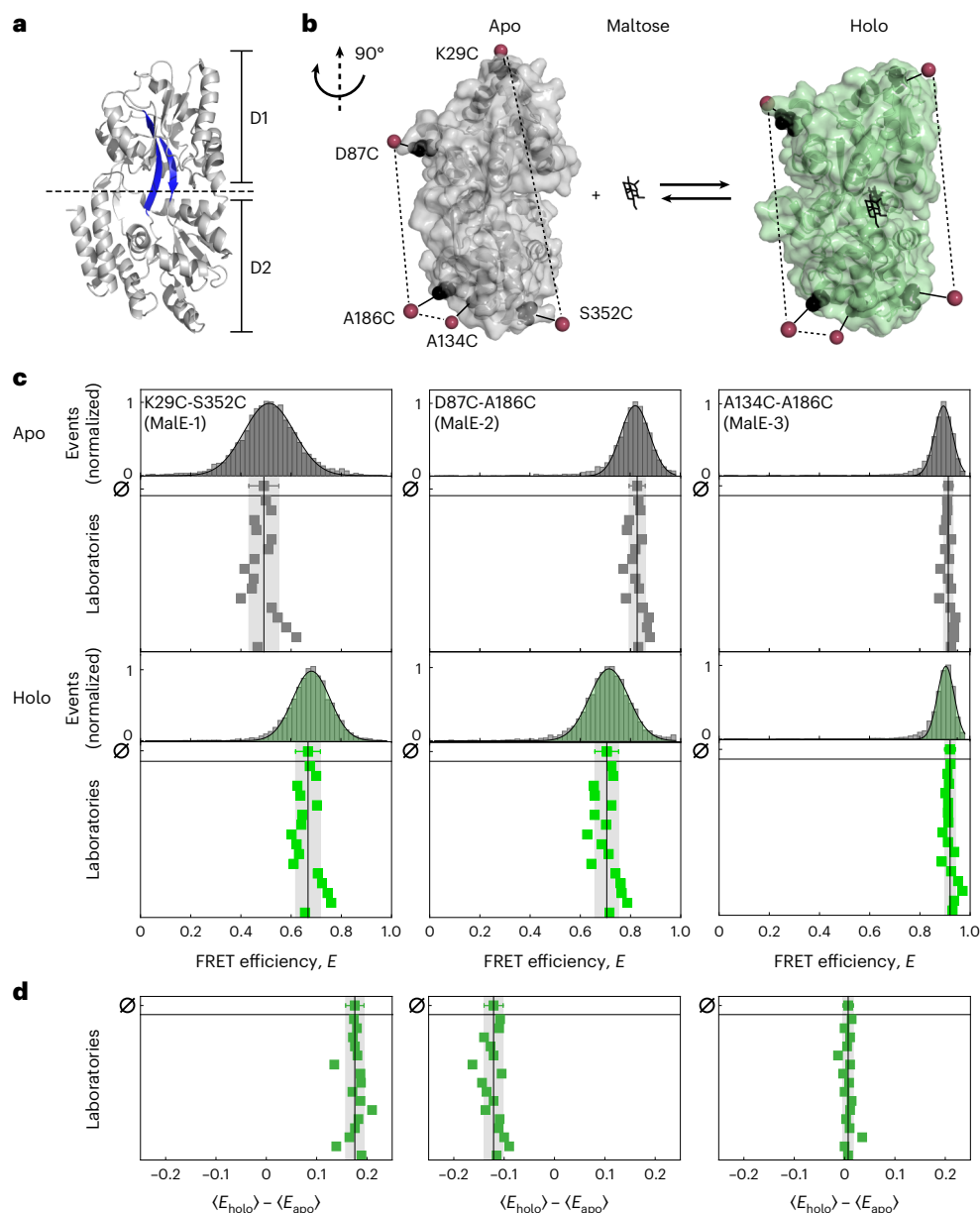
Fig. 1 | Experimental design of MalE as a protein model system for smFRET studies. a , Crystal structure of MalE in its ligand-free apo state (PDB ID 1OMP ) with domains D1 and D2 linked by flexible beta sheets (highlighted in blue). b , The crystal structure of MalE (rotated by 90° as compared to a in the apo (gray, PDB ID 1OMP ) and holo (green, PDB ID 1ANF ) states with mutations at K29C-S352C (MalE-1), D87C-A186C (MalE-2) and A134C-A186C (MalE-3) indicated in black. Note, each mutant only contains one cysteine pair and was measured using the Alexa546–Alexa647 FRET pair. The estimated mean position of the fluorophores from AV calculations are shown as red spheres. c , FRET efficiency E histograms for three MalE mutants, MalE-1 (left), MalE-2 (middle) and MalE-3 (right), in the
