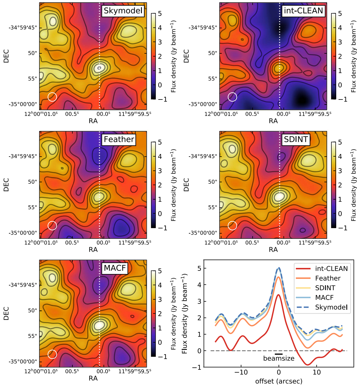
Figure 15. Compact emission recovered by different data combination methods at the central region of the sky model image convolved into a final resolution of 2'' (see bottom left corner of each image) and plotted within the same intensity range and with the same contours every 0.5 \text{ Jy beam}^{-1} . From left to right and top to bottom: sky model, int-CLEAN, Feather, SDINT, and MACF results. The bottom right panel shows the intensity profile indicated with a dotted line in our maps obtained by these methods.
