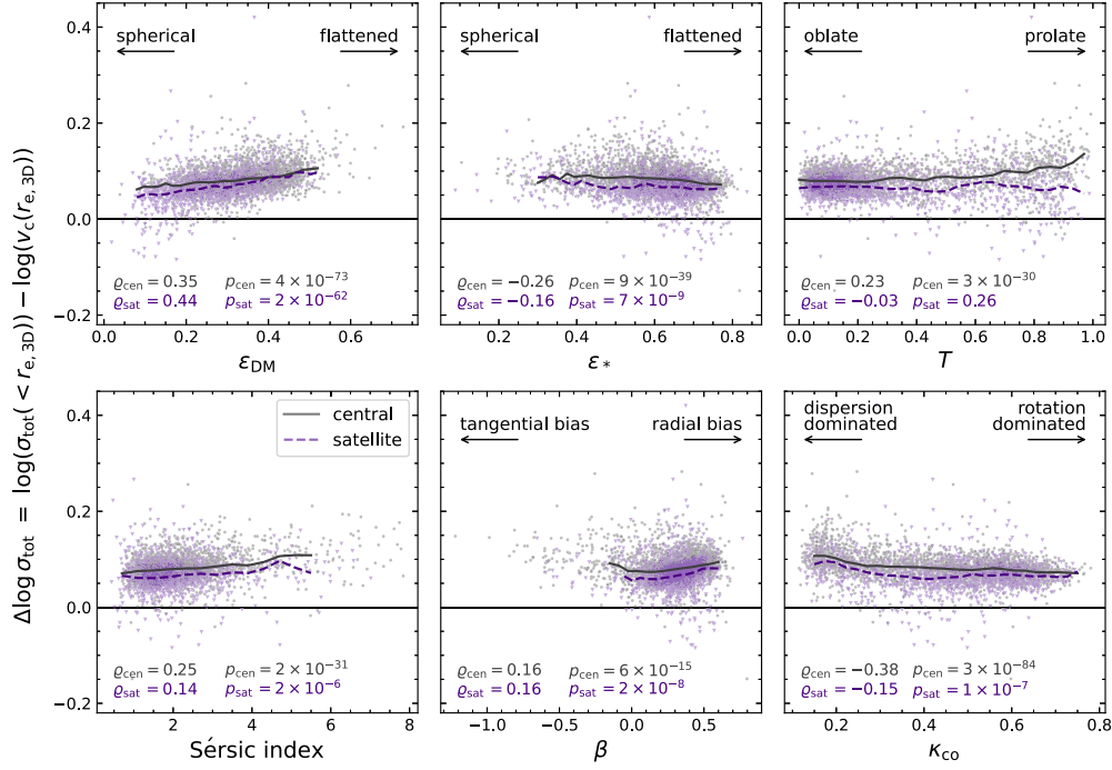
Figure 8. Deviation of the total velocity dispersion from the prediction of the virial plane (equation 11) as a function of various structural properties: the flattening of the 3D dark matter ( \epsilon_{DM} ) and stellar mass ( \epsilon_* ) distributions, triaxiality of the stellar mass ( T ), Sérsic index ( n ), anisotropy ( \beta ), and the co-rotational kinetic energy fraction ( K_{CO} ). Central (grey) and satellite (purple) galaxies are indicated separately, with solid and dashed lines showing the respective running medians in each panel. The correlations between \Delta \log \sigma_{tot} and the galaxy structure and dynamics demonstrate the effects of non-homology: galaxies have highly diverse morphologies and kinematic structures, which affects the measured value of \sigma_{tot} and hence causes a tilt in the FP with respect to the virial plane.
