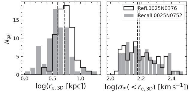
Figure A2. Probability density distribution of the 3D stellar half-mass radius (left) and the stellar velocity dispersion within this radius (right) for EAGLE galaxies of M_* > 10^{10} M_\odot . The black histogram shows the results for the 25^3 \text{ Mpc}^3 simulation run at standard resolution; the grey histogram shows the distribution for galaxies in the high-resolution simulation. The increased resolution leads to more compact galaxies, with higher Sérsic indices (Fig. A1). However, the velocity dispersions remain unchanged, and are therefore still lower than in local observations.
