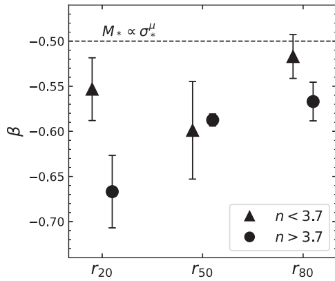
Figure 22. Tilt parameter \beta of the stellar mass FP as a function of the aperture size, for galaxies with low and high Sérsic indices in the high-resolution EAGLE simulation. The line of \beta = -0.5 implies no dependence of the stellar mass on size, i.e. the existence of a perfect TF or FJ relation. There is a weak trend towards this value of \beta for larger aperture sizes, indicating that the dark matter content plays an increasingly important role in the tilt of the stellar mass FP.
