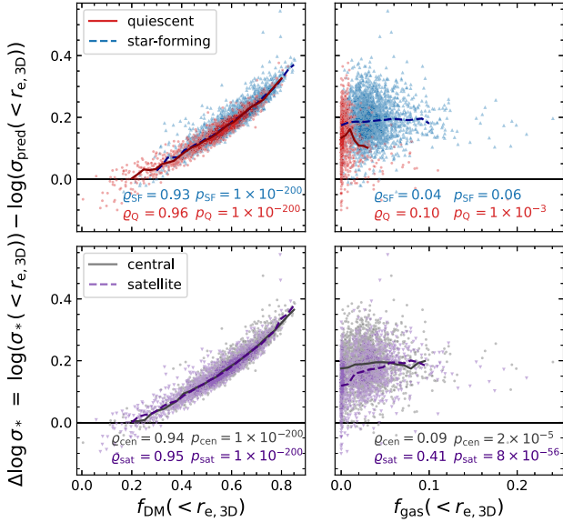
Figure 11. Deviation between the measured stellar velocity dispersion and the dispersion predicted from the stellar mass and stellar half-mass radius (equation 12; corresponding to the offset from the virial plane) versus the dark matter (left) and gas (right) fractions within the half-mass radius. Top panels distinguish between star-forming (blue) and quiescent (red) galaxies; bottom panels separate central (grey) and satellite (purple) galaxies. Solid and dashed lines show the running medians. The correlation with the dark matter fraction is stronger than for any other parameter (Fig. 9), indicating that it is the primary driver of the tilt of the stellar mass FP, for both star-forming and quiescent galaxies.
