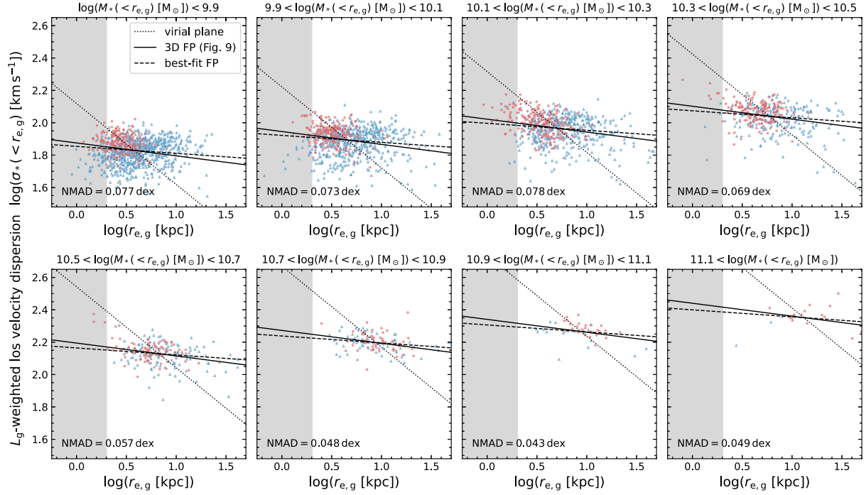
Figure C1. As Fig. 14, but using a consistent tracer (the rest-frame g -band luminosity) for both the sizes and velocity dispersions: the effective radii are measured from g -band images that do not include the effects of dust attenuation using the methodology described in de Graaff et al. (2022), and the spatially integrated stellar velocity dispersions are measured within elliptical apertures defined by these unattenuated g -band half-light radii. The strong increase in the scatter between Figs 13 and 14 is therefore not due to an inconsistency in the tracers within Fig. 14. Rather, it is the luminosity-weighting itself that causes a significant increase in the scatter.
