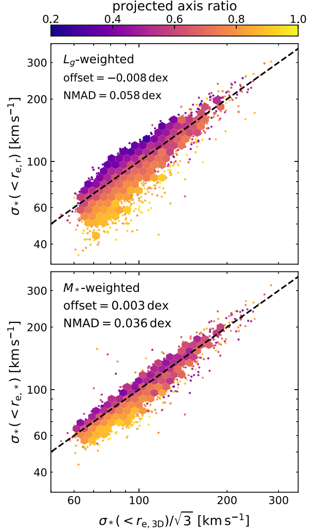
Figure 3. The spatially integrated line-of-sight stellar velocity dispersions measured in elliptic cylindrical apertures versus the 3D stellar velocity dispersion, for the luminosity-weighted (top) and stellar mass-weighted (bottom) measures. The colour coding reflects the median projected axis ratio in each bin, demonstrating that the scatter about the unit slope can be attributed mainly to projection effects and the degree to which the rotational motion along the line of sight contributes to the measured velocity dispersion.
