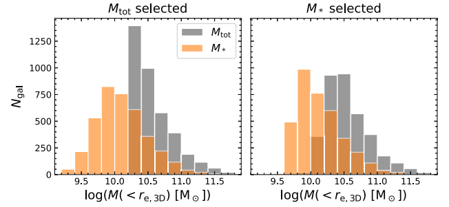
Figure 1. Distributions of the total mass and stellar mass enclosed within the 3D effective radius, for the samples selected by the total mass (left) and stellar mass (right). Total masses include all particle masses, i.e. dark matter, stellar, gas, and black hole particles.
