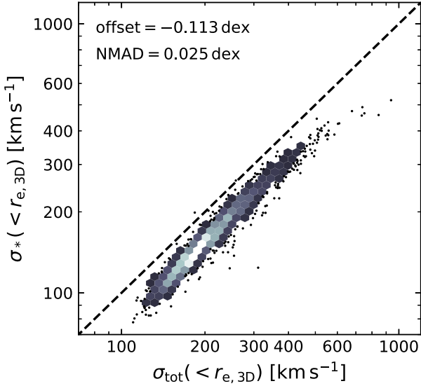
Figure 2. Comparison between the velocity dispersion of the stellar particles within r_{e,3D} and the velocity dispersion of the stellar, dark matter, and gas particles within the same aperture (equations 5 and 6). Individual data points are shown for sparsely sampled areas of the figure (created using DENSITYPLOT; Krawczyk & Peters 2014). The total velocity dispersion is greater than the stellar velocity dispersion, suggesting that the dark matter particles are dynamically hotter.
