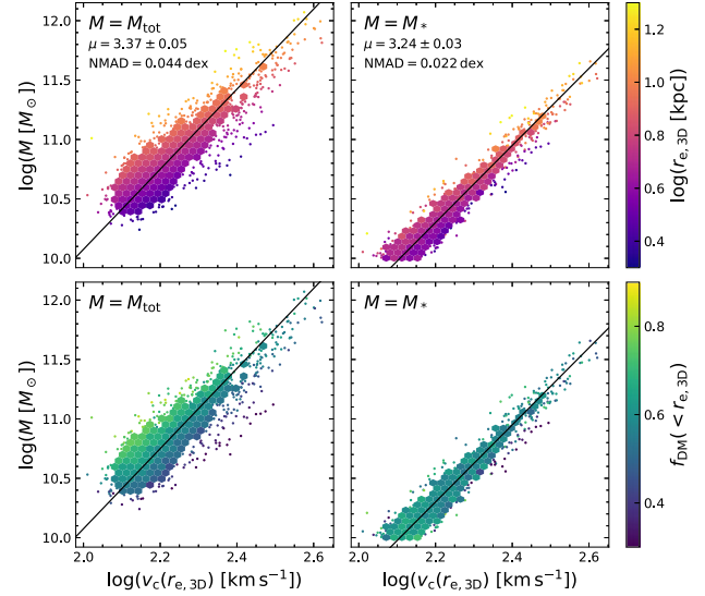
Figure 21. TF relation of star-forming galaxies, using the total mass (left) and stellar mass (right) and circular velocities calculated with equation (11). Solid lines show the relations obtained with orthogonal distance regression, and the orthogonal scatter is printed in each panel. The offset from the total mass TF relation correlates with the half-mass radius (top), and in turn also with the dark matter fraction (bottom). Because of the correlation between r_{e,3D} and f_{\text{DM}} , the stellar mass TF relation is nearly as tight as the stellar mass FP.
