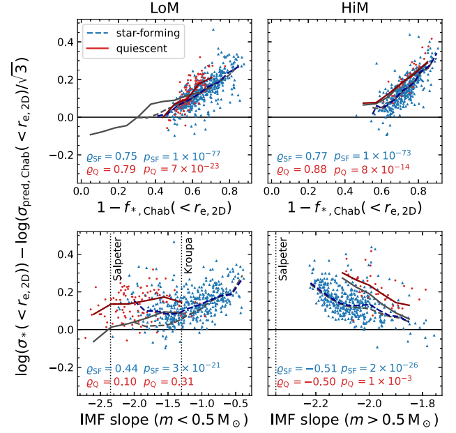
Figure 19. Deviation between the measured stellar velocity dispersion and the velocity dispersion predicted from the Chabrier-reinterpreted stellar mass for galaxies in the LoM and HiM variable IMF simulations, as a function of the dark mass fraction and luminosity-weighted IMF slope within the circular aperture of r_{e, 2D} . The Chabrier IMF underestimates the true stellar mass of galaxies in the LoM simulation, leading to increased dark mass fractions compared with Fig. 18 (grey lines show the medians from Fig. 18), and weakened correlations with the IMF slope. Galaxies in the HiM simulation are largely unaffected by a difference in the assumed IMF, which may reflect strong structural differences between galaxies in the HiM simulation and the other models.
