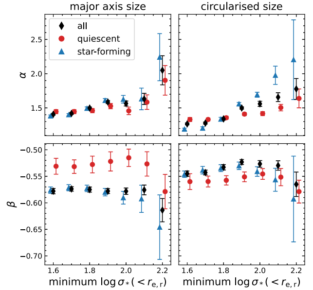
Figure 15. Effect of a selection bias in \log \sigma_* on the measured tilt of the stellar mass FP for the luminosity-weighted measurements, using the major axis effective radius (left) and circularized effective radius (right) as the measure of size. Blue and red data points have been given a slight offset in \log \sigma_* for visualization purposes. Although the \beta parameter is quite stable (varying by \lesssim 10 per cent), the \alpha parameter can vary strongly depending on the selection (differing by up to \approx 80 per cent with respect to the complete sample).
