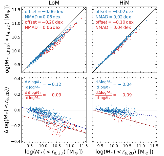
Figure 16. Comparison between the true stellar mass within the effective radius and the Chabrier-reinterpreted stellar mass, for both the LoM (left) and HiM (right) variable IMF simulations. Top panels show a direct comparison, with star-forming and quiescent galaxies indicated in blue and red, respectively. The median offset and scatter about the one-to-one relation (solid line) are printed in each panel. Bottom panels show that the difference between the two stellar masses is mass-dependent, further quantified by a linear least squares fit (dashed lines).
