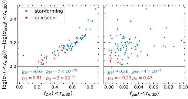
Figure A4. Deviation between the measured stellar velocity dispersion and the dispersion predicted from the stellar mass and half-mass radius (equation 12) versus the dark matter (left) and gas (right) fractions within the half-mass radius, for galaxies in the high-resolution simulation. Unlike Fig. 11, there is a weak correlation with the gas fraction for star-forming galaxies ( p -value = 0.041). However, the conclusion that the variation in f_{\text{DM}} is the primary driver of the stellar mass FP does not depend on the resolution of the simulation.
