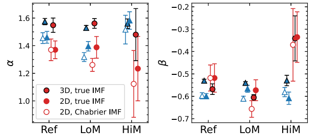
Figure 17. Measured tilt of the stellar mass FP for galaxies in the 50^3 \text{ cMpc}^3 EAGLE simulations for the reference, bottom-heavy IMF (LoM) and top-heavy IMF (HiM) models. Circles and triangles show results for the quiescent and star-forming populations, respectively. Black outlined symbols indicate the fits to the 3D aperture measurements (as in Table 1); coloured symbols show the fits to the projected measurements using the true stellar mass (filled symbols) and Chabrier-reinterpreted stellar mass (open symbols), respectively. The effects of a variable IMF are small for the intrinsic (3D) stellar mass FP. However, by assuming an incorrect IMF, the inferred tilt of the stellar mass FP can be changed by \approx 10 per cent for star-forming galaxies, and up to \approx 20 per cent for quiescent galaxies.
