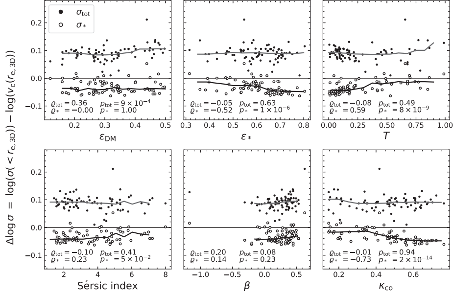
Figure A3. Analogous to Figs 8 and 9, the deviation in the total (filled symbols) and stellar (open symbols) velocity dispersion from the predicted velocity dispersion of equation (11) as a function of different structural properties, for galaxies in the high-resolution RecalL0025N0752 simulation. Lines show the running medians in each panel. Although the number of massive galaxies in the high-resolution simulation is limited, the measured correlations are similar to those found for the standard resolution. Despite a dependence of the galaxy morphology on the simulation resolution (Fig. A1), the effects of non-homology shown in Section 3.2 are not affected significantly.
