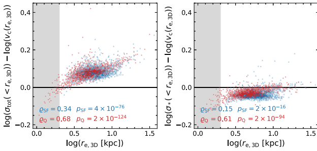
Figure 6. The offset between the FP and the virial plane, measured as the difference between the total (left) or stellar (right) velocity dispersion and the dispersion predicted by equation (11), as a function of the half-mass radius. There is not only a difference in the zero-point of the two planes, but also in the tilt: the positive Spearman rank correlation coefficients (and corresponding p-values) indicate that the FP is tilted with respect to the virial plane. This tilt is significant, and is stronger for quiescent galaxies than for star-forming galaxies.
