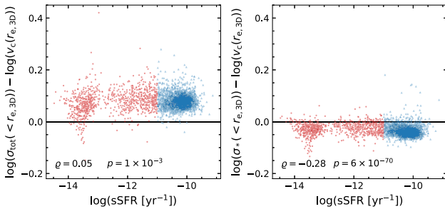
Figure 7. Difference between the measured total (left) or stellar (right) velocity dispersion and the dispersion predicted from the virial theorem (equation 11), as a function of the instantaneous sSFR. The Spearman rank correlation coefficients indicate that the sSFR has negligible impact on the deviation in \sigma_{tot} , and only a weak effect on \sigma_* .
