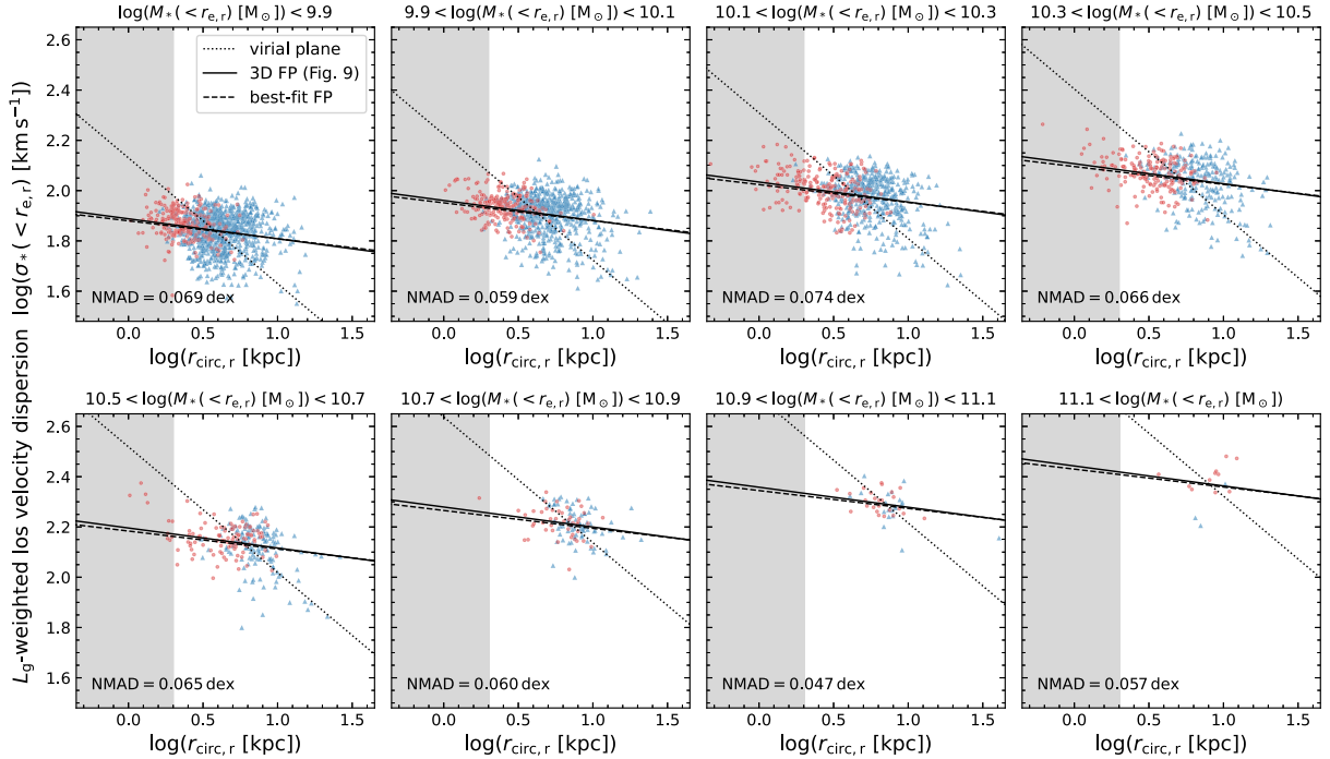
Figure B2. As Fig. 14, but showing the circularized effective radius rather than the major axis size (obtained from the best-fitting Sérsic profile to the mock r -band images).
