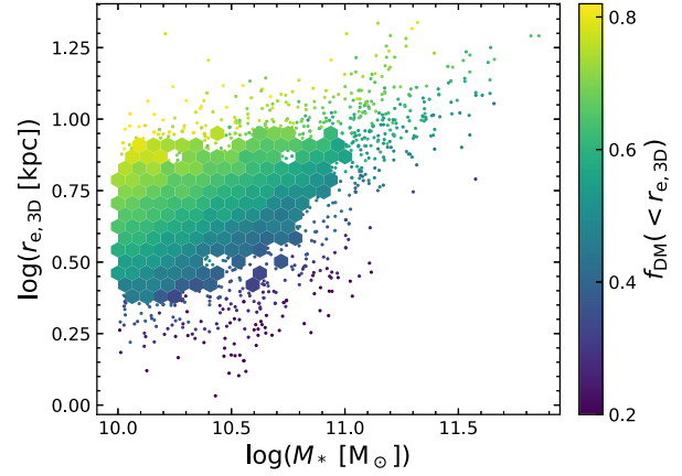
Figure 12. Total stellar mass versus the stellar half-mass radius for all (quiescent and star-forming) galaxies, colour-coded by the dark matter fraction within the half-mass radius. The variation in f_{\text{DM}} is a smooth function of both size and stellar mass, which leads to the observed correlation between \Delta \log \sigma_* and f_{\text{DM}} in Fig. 11. As a result, quiescent and star-forming galaxies lie on a common stellar mass FP that deviates strongly from the virial plane.
