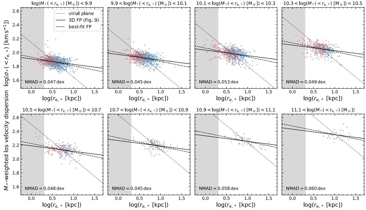
Figure 13. Stellar mass-weighted, line-of-sight velocity dispersion versus the half-mass radius from the best-fitting Sérsic profile, in bins of the stellar mass M_*( < r_{e,*}) . Star-forming and quiescent galaxies are indicated by blue and red symbols, respectively. The virial plane is shown as the dotted line, and solid lines show the stellar mass FP from fitting to the 3D aperture measurements (Table 1). The orthogonal scatter about this ‘3D FP’ is printed in each panel for comparison with Fig. 10. Projection effects and differences in the applied measurement methods result in an increased scatter, and slightly alter the inferred stellar mass FP (dashed lines; Table 3).
