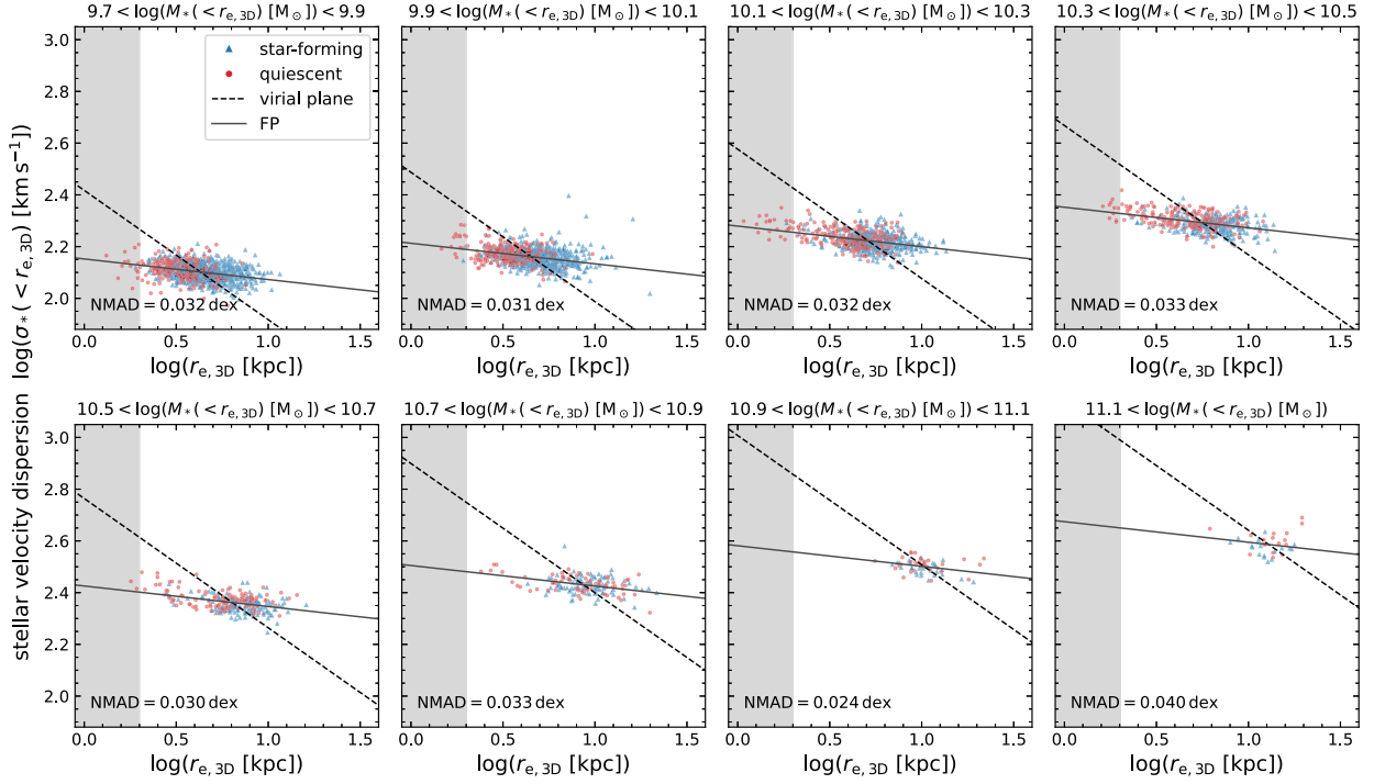
Figure 10. Stellar velocity dispersion (see Section 2.4) as a function of the half-mass radius, binned by the stellar mass M_*( < r_{e,3D}) rather than the total mass (Fig. 5). Symbols indicate the same as in Fig. 5. Galaxies clearly deviate strongly from the relations that they are expected to follow if M_{\text{dyn}} \propto M_* (dashed lines show the slope corresponding to the virial plane). In addition to the effects of non-homology established in Section 3.2, variations in the dark matter and gas fractions within r_{e,3D} must contribute to these deviations, and hence set the tilt of the stellar mass FP (solid lines).
