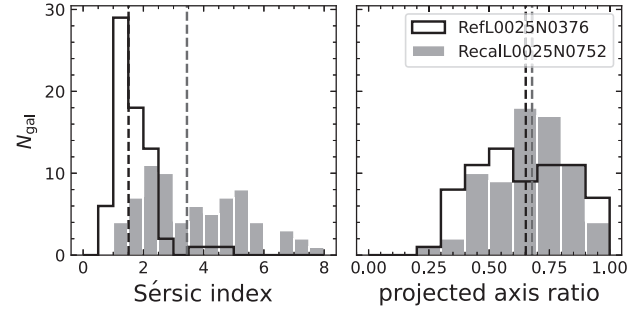
Figure A1. Probability density distribution of the Sérsic index (left) and axis ratio (right) of the projected stellar mass distribution for EAGLE galaxies of M_* > 10^{10} M_\odot . The black histogram shows the results for the 25^3 \text{ Mpc}^3 simulation run at standard resolution; the grey histogram shows the distribution for galaxies in the high-resolution simulation. The Sérsic index is strongly dependent on the resolution: the standard resolution does not produce a sufficient number of bulge-like ( n \approx 4 ) systems in comparison with observations, which is largely solved by the increased resolution. On the other hand, there is little change in the projected axis ratios, with galaxies in the high-resolution simulation being only slightly rounder.
