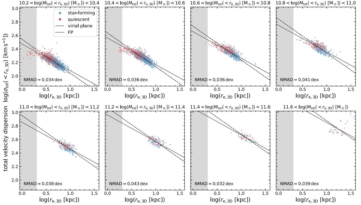
Figure 4. Velocity dispersion of all particles (dark matter, stellar, gas; see Section 2.4) as a function of the 3D half-mass radius, in bins of the total mass M_{\text{tot}}(< r_{e,3D}) . The sample is divided into star-forming (blue) and quiescent (red) galaxies by the sSFR; the grey shaded area indicates r_{e,3D} < 2 kpc, where measurements are likely to be affected by the resolution of the simulation. Dashed lines, with the intercept fit to the data in each panel, show the slope of the virial plane that galaxies are expected to follow if they are both in virial equilibrium and homologous. The best-fitting total mass FP (solid lines; Table 1) deviates slightly from the virial plane due to the effects of non-homology; the orthogonal scatter about this line is printed in each panel.
