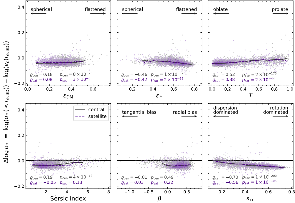
Figure 9. Deviation of the stellar velocity dispersion from the prediction of the virial plane (equation 11) as a function of galaxy structure. Compared to Fig. 8, the stellar velocity dispersion is less dependent on the shape of the dark matter distribution ( \epsilon_{DM} ), but instead depends more strongly on the structure of the stellar mass. For spherical, dispersion-supported systems \sigma_* approximates the virial plane prediction, but galaxies that are more flattened and strongly rotating diverge from this, due to the difference in the shape of the gravitational potential. Correlations are slightly weaker for satellite galaxies than centrals, which reflects the additional effect of the local environment on these systems.
