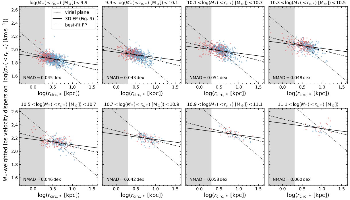
Figure B1. As Fig. 13, but showing the circularized effective radius rather than the major axis size (obtained from the best-fitting Sérsic profile to the projected stellar mass distributions).
