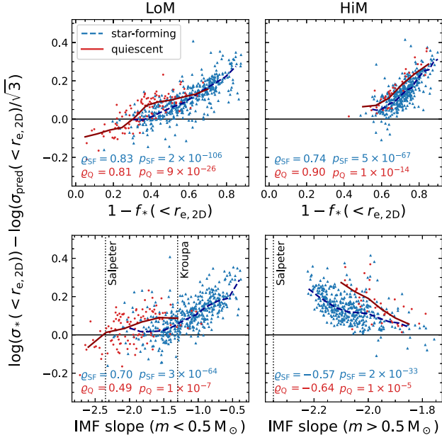
Figure 18. Deviation between the measured stellar velocity dispersion and the predicted velocity dispersion for galaxies in the LoM and HiM variable IMF simulations, as a function of the dark mass fraction and luminosity-weighted IMF slope within the circular aperture of r_{e, 2D} . Galaxies in the LoM simulation are slightly less dark matter-dominated than in the reference model (in comparison with Fig. 11), whereas the HiM model produces strongly dark matter-dominated galaxies. In both cases, there is a somewhat stronger correlation between \Delta \log \sigma_* and 1 - f_* than with the IMF slope, indicating that fluctuations in the dark matter content are the primary driver of the stellar mass FP, and likely explains the weak variation in the inferred tilt between the different simulations (Fig. 17).
