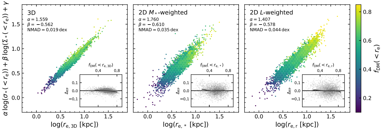
Figure 20. Edge-on view of the stellar mass FP for the intrinsic FP (relying on 3D aperture measurements; left), and the mock observed FPs using measurements weighted by the stellar mass (middle) and the observed light (right). The colour scale shows the dark matter fraction within the effective radius, and insets show the offset from the FP as a function of the same dark matter fraction. Systematic variations in f_{DM} across the galaxy population set the tilt of the stellar mass FP. The remaining scatter about the FPs anticorrelates only weakly with f_{DM} (Spearman \rho = -0.23 ), and is therefore driven by random scatter and measurement uncertainties.
