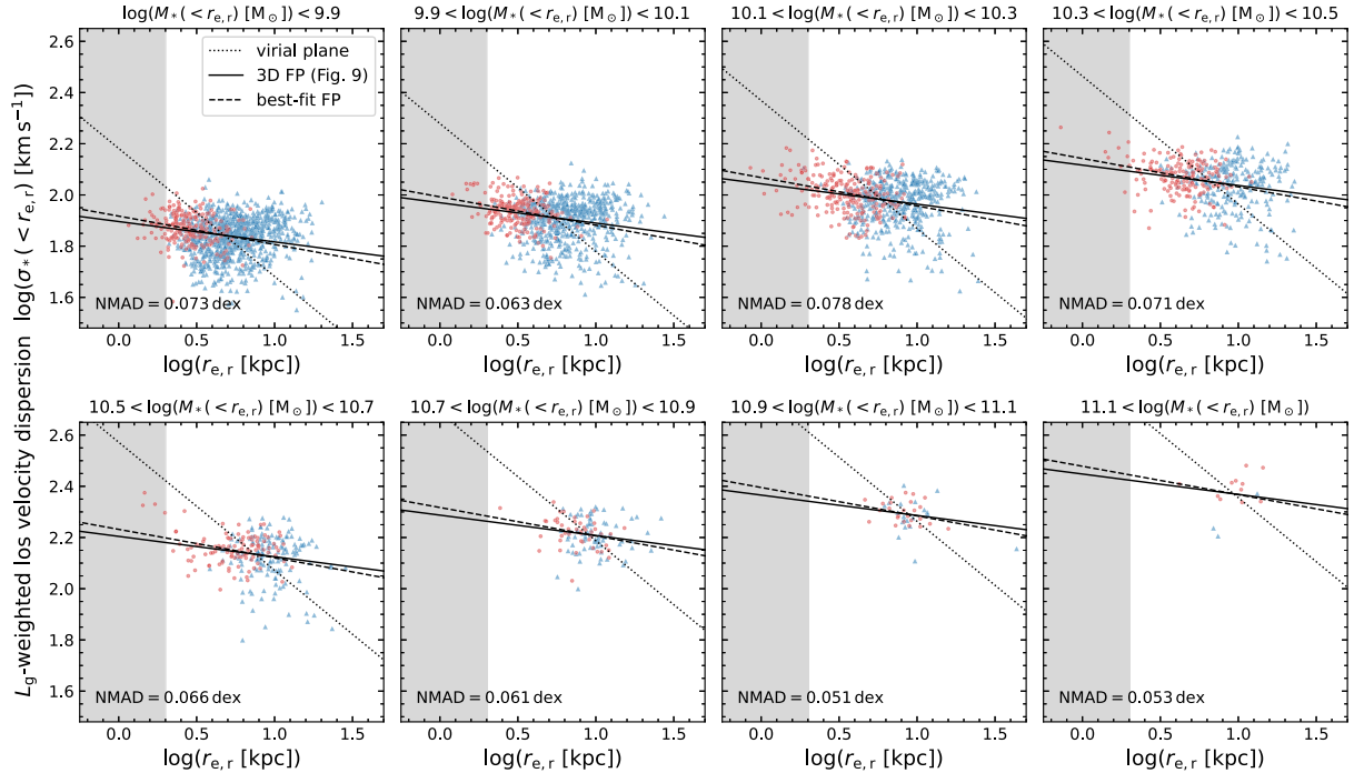
Figure 14. Projected, luminosity-weighted velocity dispersion versus the half-light radius from the best-fitting Sérsic profile, in bins of the stellar mass M_*( < r_{e,r}) . Symbols indicate the same as in Fig. 13. Gradients in the M_*/L ratio have a strong effect on the scatter, which is increased by \approx 50 per cent in the lower mass bins, and make it more difficult to precisely retrieve the intrinsic (3D) stellar mass FP.
