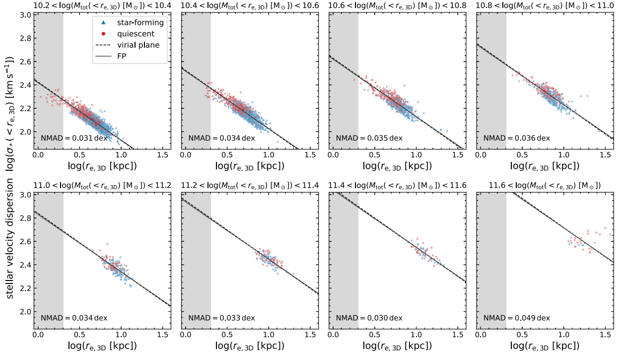
Figure 5. As Fig. 4, but showing the velocity dispersion of only the stellar particles. The scatter about the dashed lines is marginally lower, whereas the number of strong outliers (caused by recent mergers) is slightly increased. The tilt of the FP is closer to the virial plane when using \sigma_* , likely due to the decreased dependence on the galaxy structure and the fact that \sigma_{\text{tot}} is strongly influenced by the dynamically hot dark matter particles (see main text).
