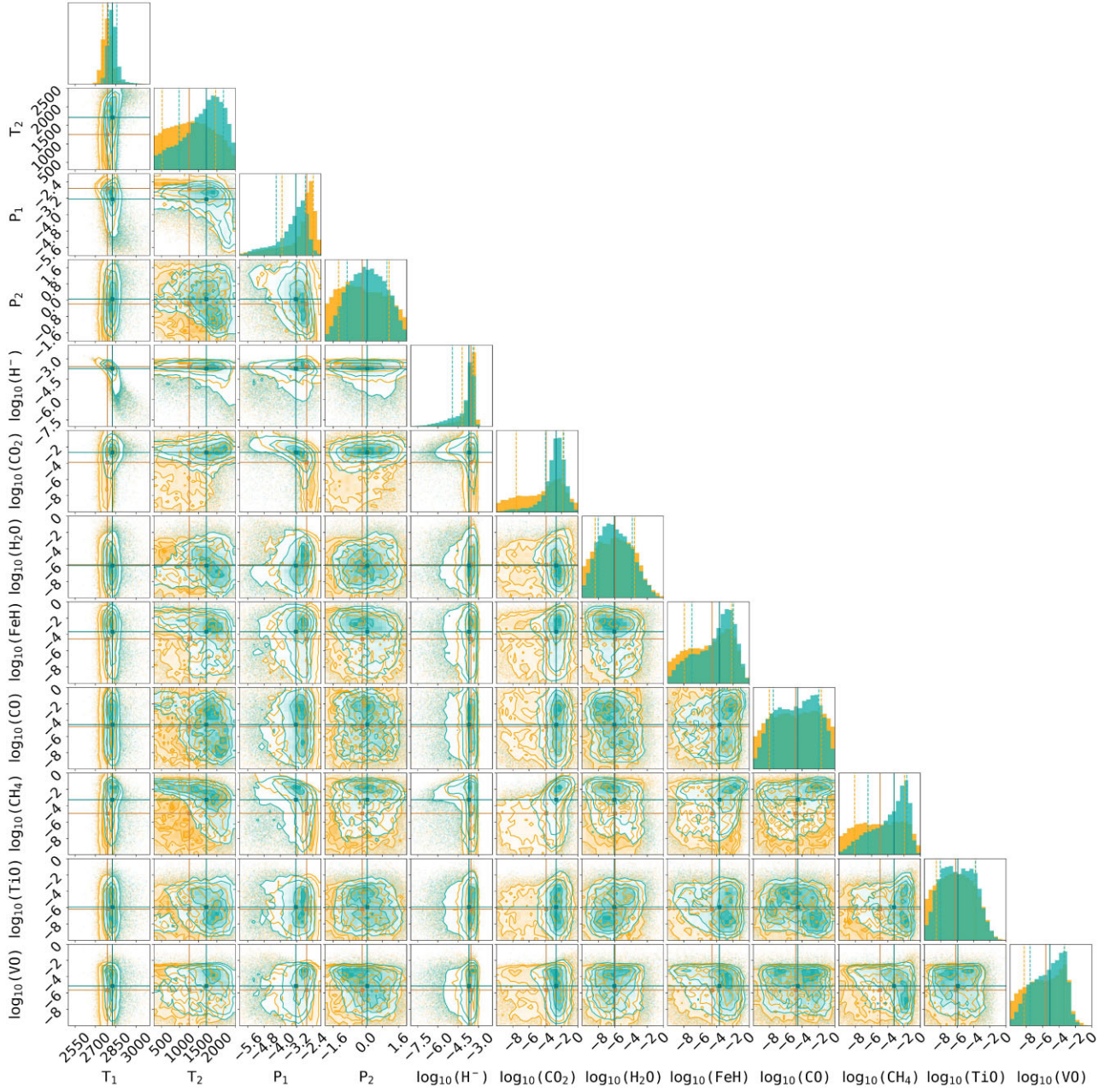
Figure A3. The retrieved atmospheric properties for the FREE retrieval on the unoffset data (green) and the 'os = -50' data (yellow) with petitRADTRANS. The orange corners represent the FREE retrieval after applying an offset of -50 ppm to the HST data.
