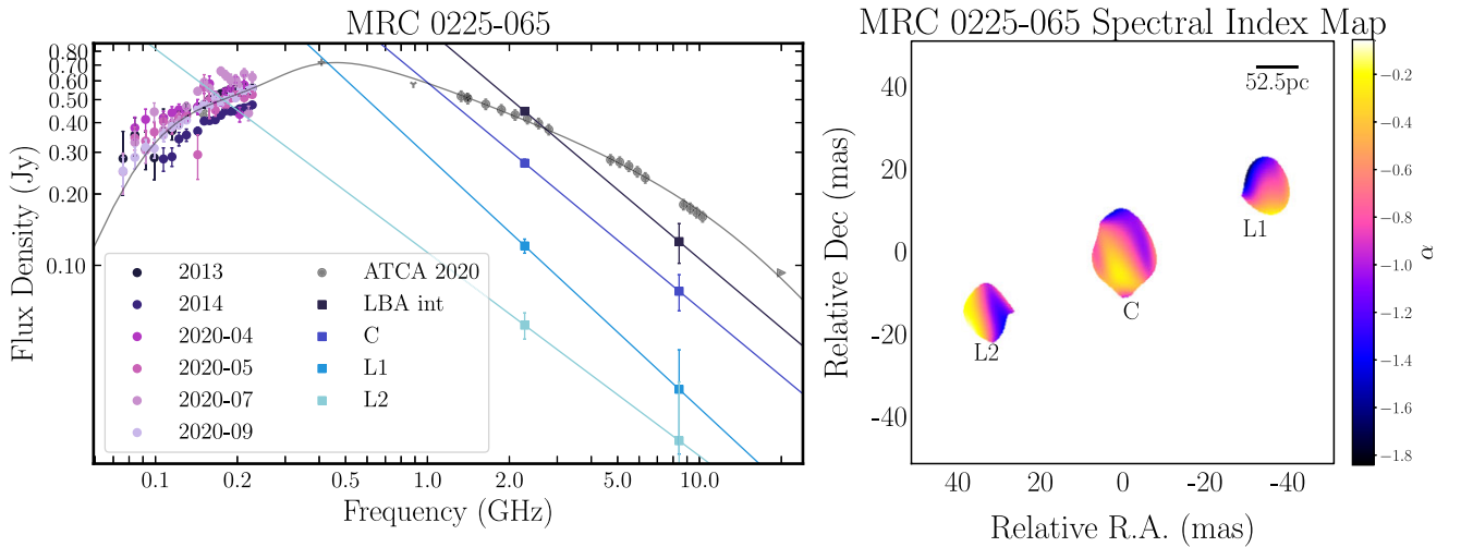
Figure 2. Spectral energy distribution (SED) for MRC 0225-065 (left) and spectral index map (right). The spectral index map was created using by convolving both the 8.3 GHz image and 2.4 GHz image to the same resolution. Data included in the SED are from R21 and R22 monitoring (circles) and coloured according to epoch. LBA flux densities are plotted as squares with the integrated flux density of LBA plotted as black squares. The spectral fit to each LBA point is a power-law with spectral index presented in Table 4. The grey spectral model to the entire SED is a double SSA model with an exponential break. Supplementary data included: TIFR GMRT 150 MHz Sky Survey Alternative Data Release 1 (TGSS-ADR1; Intema et al. 2017) (grey cross), Molonglo Reference Catalogue (MRC; Large et al. 1981; Large, Cram, & Burgess 1991) (grey +), Rapid ASKAP Continuum Survey (RACS; McConnell et al. 2020; Hale et al. 2021) (grey 'Y'), NRAO VLA Sky Survey NVSS; (NVSS; Condon et al. 1998), Australia Telescope 20 GHz (AT20G; Murphy et al. 2010) (grey right arrow).
