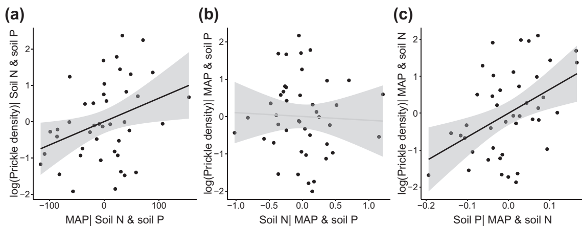
Figure 2. Variation in prickly density along gradients of (a) rainfall, (b) soil N, and (c) soil P represented as partial residual graphs, i.e. covariation due to other variables in the model are already accounted for. In the figure, each dot is the residual of log transformed mean prickly density at a site, dark lines represent significant relationships and grey lines represent insignificant relationships based on univariate models, and grey areas represent the 95% confidence intervals.
