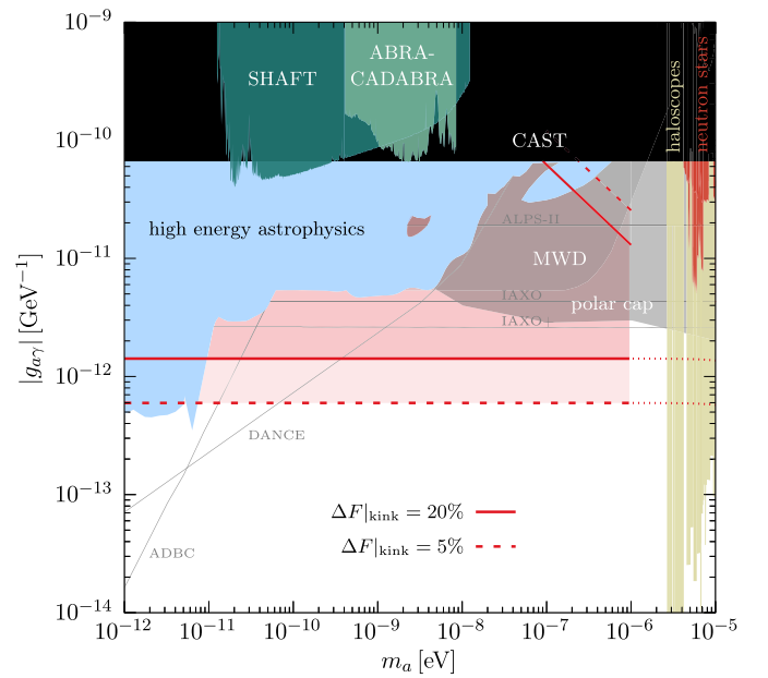
Fig. 3. Sensitivity region on photon-ALP resonant conversion bounded by the solid (dashed) red line based on the assumption that a 20% (5%) spectral feature can be detected. Astrophysical constraints are cumulatively shown by the blue shaded region labeled “high energy astrophysics” (see [76]) from magnetic white dwarfs (MWD) [77] and pulsar polar caps [78]. Laboratory limits from CAST [79], SHAFT [80], ABRACADABRA [81] and projections for ALPS-II [82], IAXO(+) [83], DANCE [84], and ADBC [85] are shown as labeled. Additional constraints that assume ALPs being DM are from haloscopes [86–92], previous analyses using neutron stars [42,43,46], or axion stars [93].
