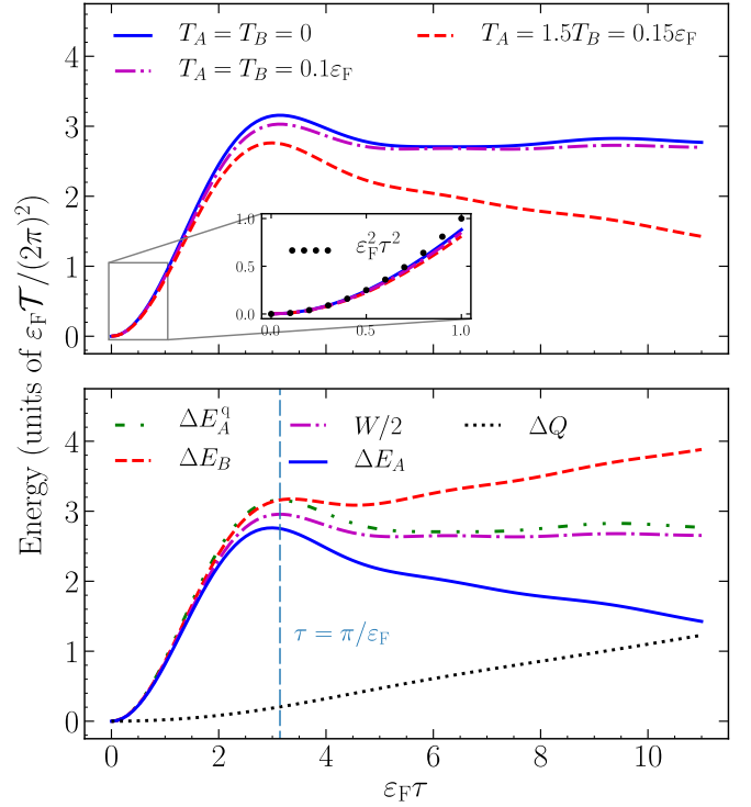
FIG. 1. (Top) Energy increment in reservoir A , \Delta E_A , due to quench-coupling with B as a function of time calculated from Eq. (9). The inset demonstrates that the approximation of \tau \ll 1/\varepsilon_F in Eq. (10) accurately describes the energy increment up to \tau \sim 1/\varepsilon_F for a given initial temperature imbalance. (Bottom) Energy balance in the system upon decoupling at t = \tau for T_A = 0.15\varepsilon_F and T_B = 0.1\varepsilon_F . \Delta E_A^q is the energy change at zero temperature (10), \Delta E_B is the energy change in the initially colder system, W is the work done by the quench upon decoupling, and \Delta Q is the heat transferred from A to B . The vertical line marks the maximum of \Delta E_A^q . The figures for a different set of initial temperatures are presented in the Supplemental Material [42].
