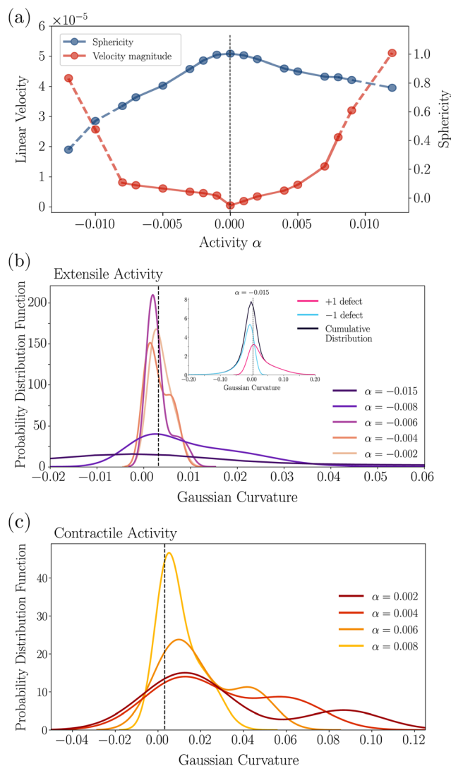
Fig. 3 Flattening and defect-curved coupling for polar LC. (a) The shell's speed and sphericity for different activities. We observe that the sphericity remains larger as contractile activity is increased, compared with the situation for increasing extensile behavior. To better quantify our observation and justify our claim, that active defects flatten the sphere for extensile activity we consider the probability density function of the position of defects as a function of the local Gaussian curvature for different activities. (b) Probability distribution of the Gaussian curvature for extensile activity. The Gaussian curvature of the undeformed sphere of radius R_0 = 18 is given by K \approx 0.003 and indicated by the dashed line. Indeed, in this case defects (vortex) are more likely to be found in flat regions and the probability distribution function is peaked near zero Gaussian curvature. The inset shows the probability distribution of the Gaussian curvature for the case \alpha = -0.015 , that is in the active turbulence regime. We present the curves for positive (magenta) and negative (cyan) defects, as well as their sum (black). On the other hand, in (c), defects in the presence of contractile activity (aster) are more likely to be found in regions where the local Gaussian curvature is greater than that for an undeformed sphere.
