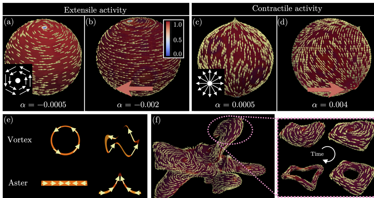
Fig. 2 Active polar LC on elastic shell. (a–d) Typical configuration of active shells and polar LC arrangements for extensile activity, panels (a and b), and contractile activity, panels (c and d). The yellow vectors denote the local direction \mathbf{p} polarization field whose magnitude \Psi_1 is used to color the shell surface according to the color bar in (b). (a) For small extensile activity ( \alpha = -0.0005 ) defects (blue) with the local geometry of a vortex (sketched in inset) are located at the poles of an undeformed sphere and create an azimuthal flow. In (b), for larger extensile activity ( \alpha = -0.002 ), the sphere flattens and the defects move away from the poles to increase the bending instability of the director field. This symmetry breaking results in the shell moving in the direction of the red arrow. (c) On the other hand, in the case of small contractile activity ( \alpha = 0.0005 ) we observe buckling near the aster-shaped defects (aster sketched in inset). (d) Similarly as for extensile activity, for larger contractile activity ( \alpha = 0.004 ), the two aster-like defects move away from the poles and the shell becomes motile. (e) To phenomenologically illustrate why we observe buckling only for asters but not for vortices, we sketch the escape in the third dimension for a LC coupled to an elastic ribbon. The aster configuration (bottom) is able to escape with significantly less deformation of the ribbon (right column) than for the vortex (top). The yellow arrows represent the orientation of the polar liquid crystal and the orange ribbon the confining substrate. (f) Deformed shell in the turbulent extensile regime ( \alpha = -0.015 ). The region circled in pink produces a vesicle that eventually transforms from a flattened sphere to a torus, as shown in the time-series on the right. The hole of the torus increases in time and eventually the torus rips apart into a filament. The parameters used in all simulations can be found in the Appendix A.3.
