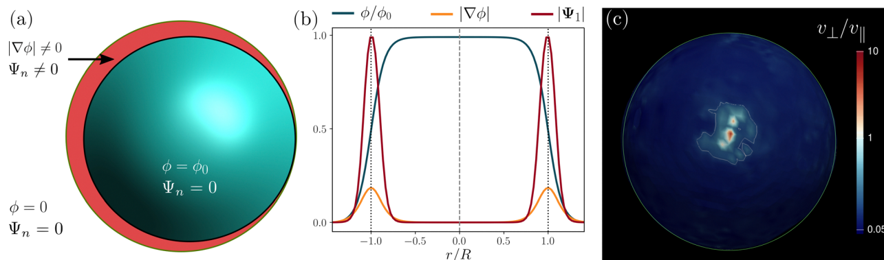
Fig. 7 (a) Cross-section of an active shell, as modeled in our numerical simulations. In the interior of the droplet (plotted in green) \phi = \phi_0 , while \phi \approx 0 in the exterior. Concentration gradients \nabla\phi are significant only at the droplet interface (red in the picture). By construction the orientational order parameter \Psi_n is finite when |\nabla\phi| is larger than a critical threshold (see Appendix A), hence the fluid is orientationally ordered and active within a thin shell which corresponds to the droplet interface and isotropic as well as passive elsewhere. (b) The radial profiles (with r being the distance from the centre of the droplet) measured from simulations and expressed in lattice units of \phi , \nabla\phi and the magnitude of the order parameter |\Psi_1| for the polar case. Panel (c) shows the color-plot of the ratio of normal versus tangential flow v_\perp/v_\parallel measured in simulations for the polar case of Fig. 1(b). Notice that normal flows are significant only in proximity of topological defects.
