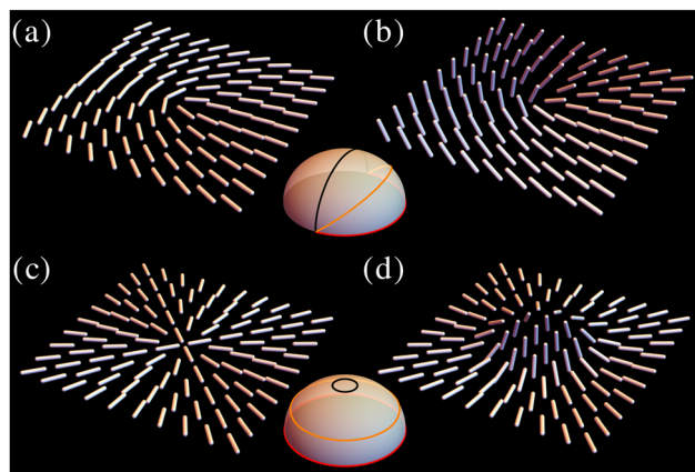
Fig. 4 Topological protection of nematic defects. (a) Configuration of a +1/2 defect on the plane. (b) A +1/2 disclination can be continuously deformed into a -1/2 disclination upon rotating the director about an arbitrary axis on the plane of the director by an angle \theta = \pi . By contrast, rotating the director by an angle \theta = \pi/2 gives rise to an escaped-like configuration, but does not remove the central singularity, which is, therefore, topologically protected. The latter can be better appreciated by considering the corresponding trajectory traced by the director in one loop around the defect core and corresponding to a hemicycle connecting two antipodal points on the hemisphere (inset). These, in turn, correspond to the same orientation in the physical space because of the D_{\infty h} symmetry of uniaxial nematics. In this representation, semi-integer point defects correspond to hemicycles on the equatorial plane (red curve), with their sign given by the orientation of the hemicycle with respect to that of the equator. Escaped-like configurations correspond instead to hemicycles connecting two antipodal points across the positive half-space (orange and black curve), while an isolated point identifies a uniformly oriented configuration. Whether lying on the equatorial plane or bending across the positive half-space, hemicycles cannot be contracted into a point, thus it is impossible to continuously transform a planar disclination into a defect free configuration by rotating the nematic director out of plane. (c) Configuration of a +1 defect on the plane. (d) Unlike for semi-integer defects, a +1 planar disclination can be continuously transformed into a defect free state upon rotating the director perpendicularly to the plane. In the order parameter space, this amounts to contracting a loop around the equator into a point (inset).
