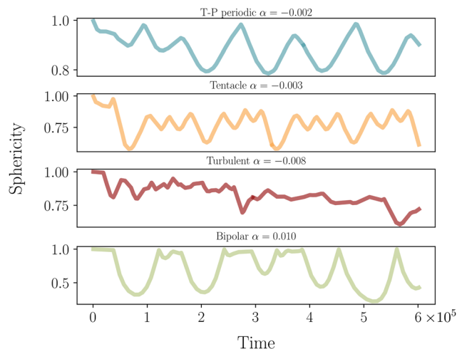
Fig. 6 Periodic deformation of elastic shell. To quantify the periodic deformation of the sphere due to the active nematic defects we show the sphericity of the elastic shell as a function of time in panel for different values of activity. Each of the activity values we chose corresponds to one of the four different phases we found (see Fig. 5). The periodicity in the sphericity is clearly visible, as is the fact that the deformation increases with increasing activity.
