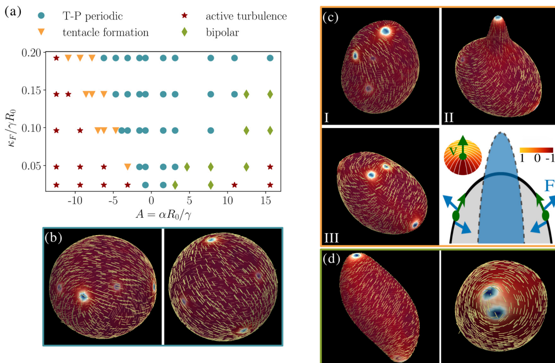
Fig. 5 Active nematic LC on elastic shell. We observe four distinct phases for an active nematic liquid crystal as presented in the phase diagram in (a). At small activity +1/2 -defects move periodically on an essentially undeformed sphere (blue circles, tetrahedral–planar (T–P) periodic). Defects oscillate between a planar (left snapshot in panel (b)) and a tetrahedral (right snapshot in panel (b)) configuration. For larger extensile activity, defects deform the sphere periodically and, for sufficiently large activity, protrusions are formed (yellow triangles in (a)) as shown in (c) for \alpha = -0.003 . In the main text, using the sketch in (c), it is explained how the pressure field of a +1/2 -defect moving with velocity \mathbf{v} (top-left corner) can lead to a dipolar normal force \mathbf{F} (blue arrows in the sketch) that creates the protrusion. For larger contractile activity we observe a bipolar configuration (green diamonds in (a)) as shown in (d), for \alpha = 0.002 , with two +1/2 defects located near each pole. For even larger activity we find a turbulent regime (red stars).
