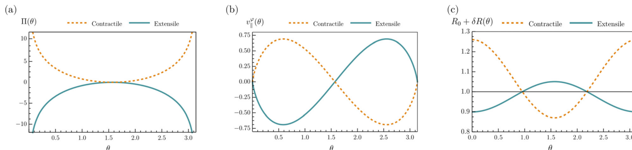
Fig. 8 In panels (a and b) we show, respectively, the pressure \Pi (eqn (S23)) and physical velocity field v_\phi^p(\theta) (eqn (S26)) multiplied by \sin \theta for a fixed sphere for contractile and extensile activity. In panel (c) we show the radius of the deformed sphere for extensile and contractile activity, see eqn (S38). The black horizontal line corresponds to \delta R(\theta) = 0 . If the extensile activity is sufficiently large, as it is here, the sphere flattens at the poles, that is the radius after deformation is less than R_0 . The parameter values used for all panels are \alpha = \pm 5 , \lambda = 1.1 , \eta = 1 , \kappa_F = 1 , \gamma = 1 , \kappa_B = 1 , R_0 = 1 .
