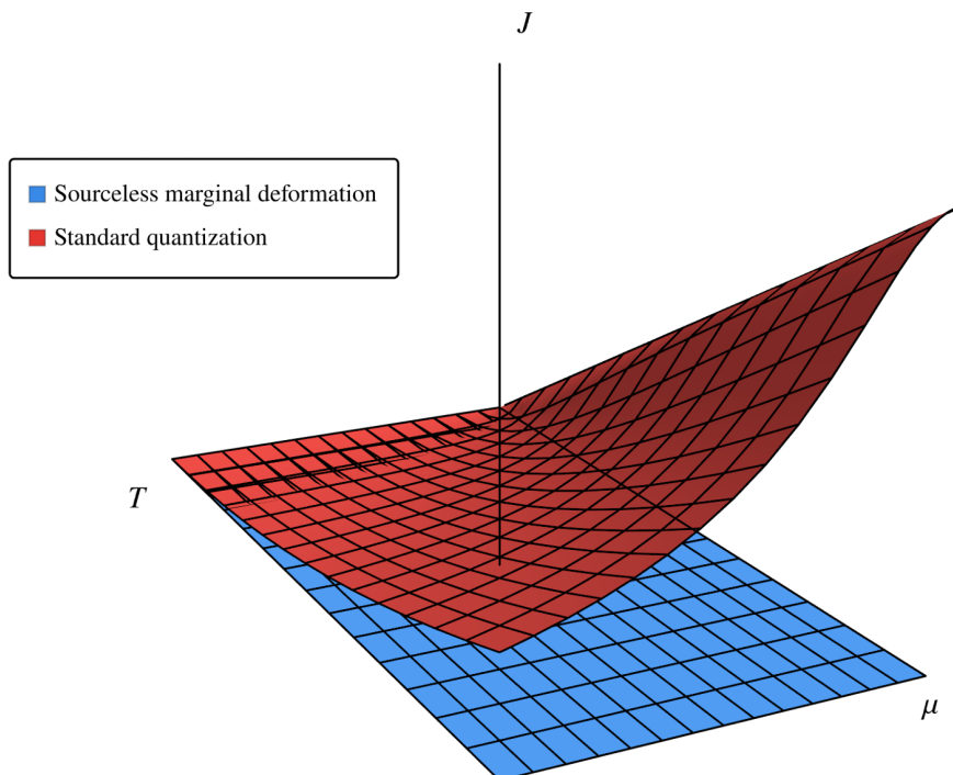
Figure 1. aGR solution manifold in the thermodynamic parameter space of source \{T, \mu, J\} for two specific choices of boundary interpretations (cases (i) and (ii)). The sourceless marginal case has trivial source and is by itself a 2-charge submanifold while the standard quantization case has a constrained source which leads to the non-trivial corrections in s_1, \rho_1 .
