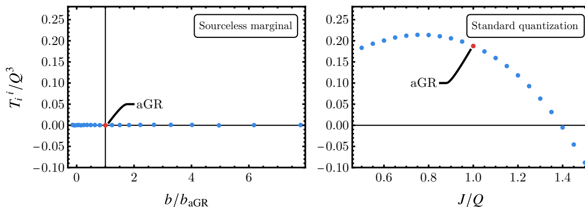
Figure 3. Trace of the boundary stress tensor when varying the Dirichlet boundary condition \psi(0) . This can be interpreted as exploring boundaries with a = 0, J = 0 and varying marginal coupling b (left) or as changing the source J = \alpha in standard quantization (right). aGR denotes the analytically known Gubser-Rocha solution. (Left) We see that in this case, T_{ij} remains traceless regardless of b which is consistent with a marginal deformation and the result (3.16). (Right) In standard quantization, the trace is generically not zero, but this can happen for specific boundary theories: sourceless J = 0 — not visible on the graph — and when \mathcal{O}_\varphi = 0 — which happens at J/Q \simeq 1.4 .
