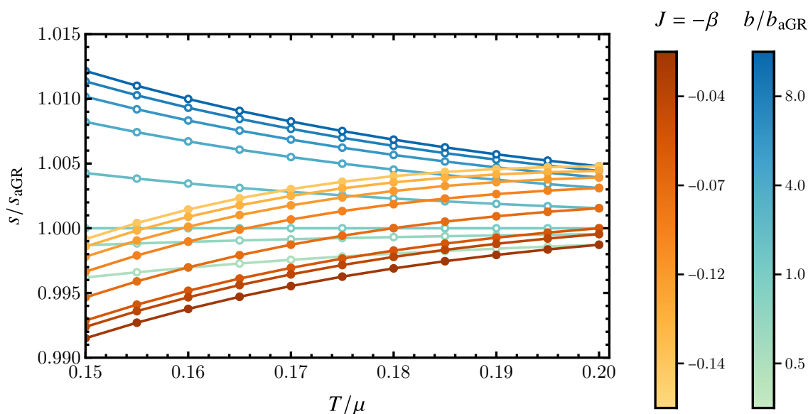
Figure 5. Black hole entropy as a function of T/\mu when keeping either the alternate quantization source J = -\beta fixed (choice 3, orange gradient curves) or when keeping the label b(\psi(0)) fixed (choice 1, blue gradient curves). The curves meet in pairs at T/\mu = 0.20 — indicating identical bulk solutions — and separate for other temperatures — indicating different black hole solutions.
