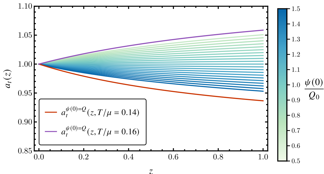
Figure 2. Gauge field component a_t(z) as defined in (4.1) at T_0/\mu = 0.15 and for various values of \psi(0) . We compare with the equivalent function a_t^{\psi(0)=Q} of the aGR solution at different temperatures T/\mu = 0.16 (purple) and T/\mu = 0.14 (red). This illustrates that qualitatively the effect of changing the dilaton boundary value has similarities to changing the ratio T/\mu .
