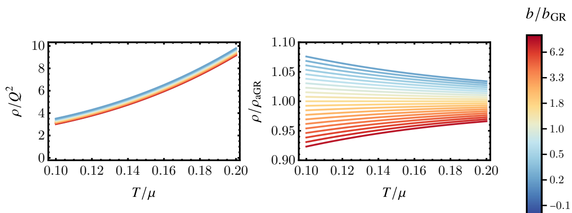
Figure 4. Boundary charge density as a function of the temperature T/\mu when imposing Dirichlet boundary conditions, which we interpret as varying the boundary theory through b . The charge density is normalized by Q^2 in the left-hand plot and by its aGR value defined in (3.24) in the right-hand plot. The qualitative behaviour of all these theories is extremely similar to the aGR solution (left) but quantitatively differs as a function of T/\mu (right), showing the theories described are different.
