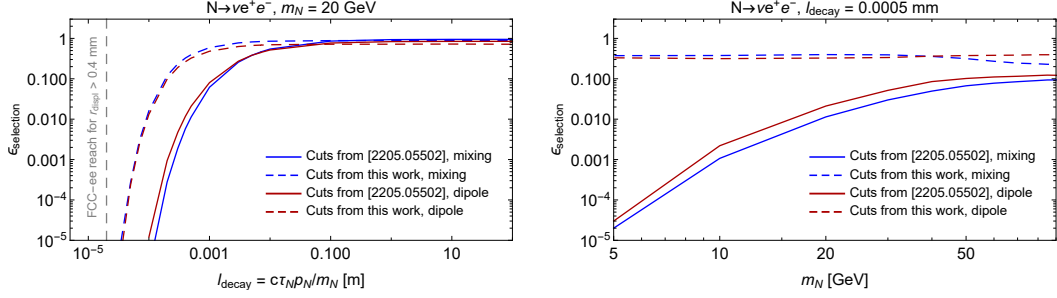
Figure 7. Selection efficiency for the process N \rightarrow e^+ e^- \nu (for both the mixing and dipole couplings) based on the cuts from table 3: the ones considered in [52] (the blue lines), and the ones discussed in this work (the red lines), assuming the minimal displacement l_{\text{displ}} > 0.4 mm. The left panel: as a function of the HNL decay length l_{N,\text{decay}} = c\tau_N p_N/m_N for the fixed HNL mass m_N = 30 GeV. The vertical dashed gray line denotes the minimal decay length of the HNL with the mixing coupling to which FCC-ee may be sensitive if requiring only the displacement r_{\text{displ}} > 0.4 mm (from [52]). The right panel: as a function of the HNL mass for the fixed HNL decay length l_{N,\text{decay}} = 0.5 mm.
