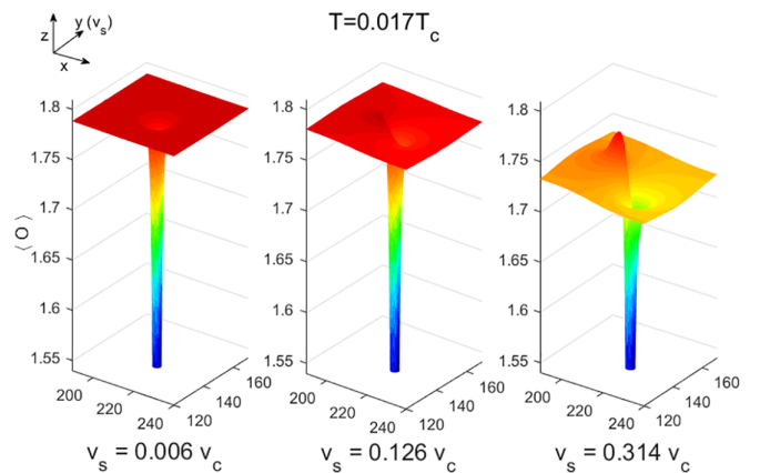
FIG. 10. Order-parameter profile of the vortex in the stationary long time regime as function of increasing drives v_s = 0.006v_c , 0.126v_c , and 0.314v_c , respectively. For the largest current case, it is evident that the background order parameter was becoming smaller, as the system began to approach the critical current.
