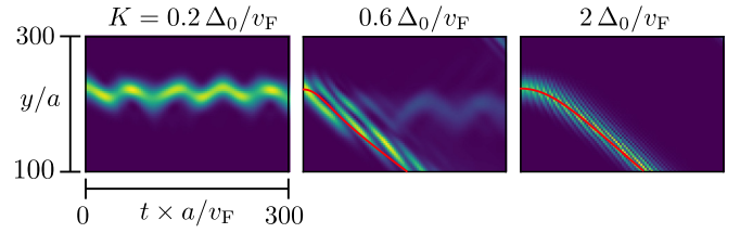
FIG. 4. Propagation of the zero-mode along the y axis after the superflow momentum quench at t = 0 . The color scale shows the density profile \int |\Psi(x, y, t)|^2 dx following from the computer simulation ( \Delta_0 = 0.2 v_F/a , r_0 = 40 a , B = (h/e)(302 a)^{-2} ). The red curve results from integration of the semiclassical equation of motion (4.10), for the same \Delta(r) = \Delta_0 \tanh(r/r_0) gap profile as in the numerics [24].
