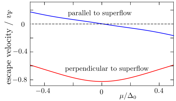
FIG. 8. Dependence of the direction of the escape velocity on the chemical potential \mu (for fixed \Delta_0 = 0.2 v_F/a , K = 2\Delta_0/v_F , and vortex core size r_0 = 40 a ).
