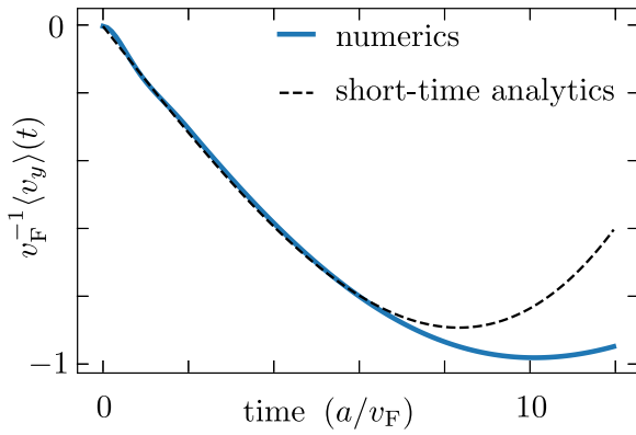
FIG. 6. Initial time dependence of the expectation value of the velocity v_y of the Majorana wave packet (perpendicular to the superflow), for \Delta_0 = 0.04 v_F/a , K = 2\Delta_0/v_F , in the limit r_0 \rightarrow 0 of a small vortex core. The dashed curve is the analytical result from Eq. (3.6).
