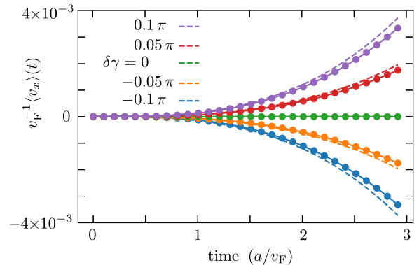
FIG. 9. Dependence of the velocity v_x parallel to the superflow on the phase shift \gamma = \pi/4 + \delta\gamma between the electron and hole components of the initial wave packet (for \Delta_0 = 0.04 v_F/a , K = 2\Delta_0/v_F , r_0 \rightarrow 0 ). This is data for \mu = 0 , the deflection in the x direction happens when \gamma is pushed away from \pi/4 by an initial voltage pulse. The solid curves are numerical results, the dashed curves are the short-time analytics (3.5).
