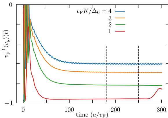
FIG. 7. Time dependence of the velocity when the Majorana wave packet is driven out of the vortex core by the Magnus force. Four values of the superflow momentum K are shown at fixed \Delta_0 = 0.2 v_F/a . The average over the time interval between the dashed lines is the escape velocity plotted in Fig. 5 (green curve, for r_0 = 20 a ). For much shorter times the wave packet is still trapped in the vortex core. For longer times the wave packet reaches the boundary of the magnetic unit cell.
