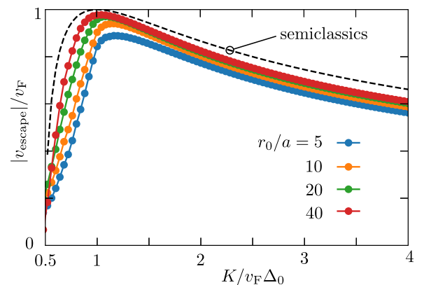
FIG. 5. Escape velocity of a zero-mode wave packet from the vortex core, as a function of the superflow momentum K . The data points follow from the computer simulation, for different core sizes r_0 (at fixed \Delta_0 = 0.2 v_F/a ). The black dashed curve is the semiclassical result (4.9).
