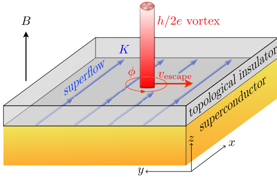
FIG. 1. Schematic of a topological insulator with induced superconductivity (gap \Delta_0 ) in a perpendicular magnetic field B . A vortex (red, with a 2\pi winding of the superconducting phase \phi ) binds a Majorana zero-mode. An in-plane supercurrent (blue arrows, Cooper pair momentum K ) can deconfine the zero mode, producing a Majorana fermion wave packet that escapes with velocity v_{\text{escape}} in a direction perpendicular to the superflow.
