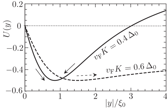
FIG. 3. Plot of the potential U(y) that governs the equation of motion (4.10) of the wave packet, calculated for the gap and superflow velocity profiles (4.11). The arrows indicate the oscillatory motion for v_F|K| < \Delta_0/2 and the escape to infinity for v_F|K| > \Delta_0/2 . The direction in which the wave packet escapes is minus the sign of K times the sign of the vorticity.
