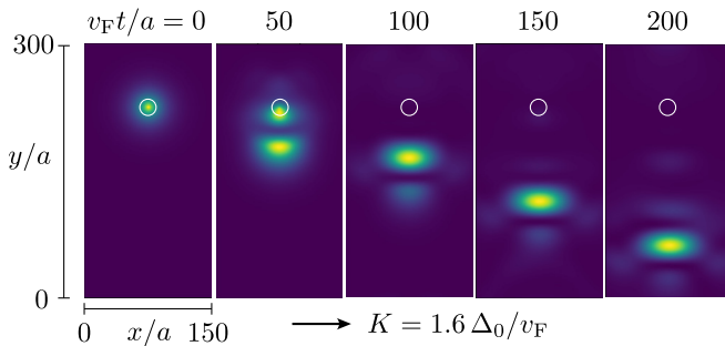
FIG. 2. Majorana fermion wave packet that escapes from a vortex (white circle) in response to a quench of the superflow momentum K (in the x direction). The images show a color scale plot of |\Psi(x, y, t)|^2 in the plane of the superconductor, at different times following the quench at t = 0 . This is a numerical solution of the evolution equation (2.6), with Hamiltonian (2.5) discretized on a square lattice (lattice constant a , \Delta_0 = 0.04 \hbar v_F / a , B = (\hbar/e)(302a)^{-2} , \mu = 0 ). The initial condition at t = 0 is the Majorana zero mode \Psi_+ . For a full animation of the wave packet see, Supplemental Material [14].
