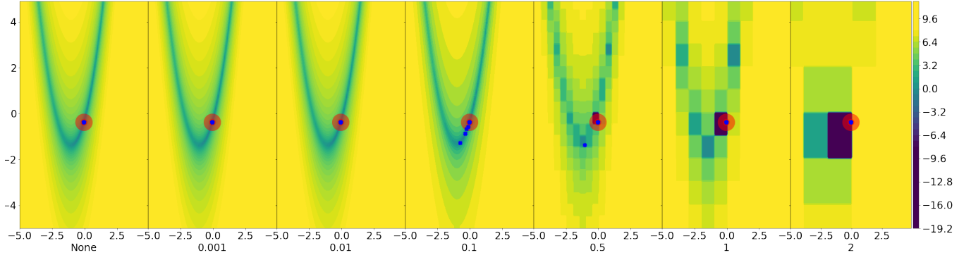
Figure 9: 2D plot of the landscape for F8 (Rosenbrock) for different plateau sizes \rho \in \{\text{None}, 0.001, 0.01, 0.1, 0.5, 1.0, 2.0\} . The red circle shows the location of the solution and the blue crosses are the best points found by CMA-ES (indicating the plateau, not the exact location seen by the algorithm itself).
