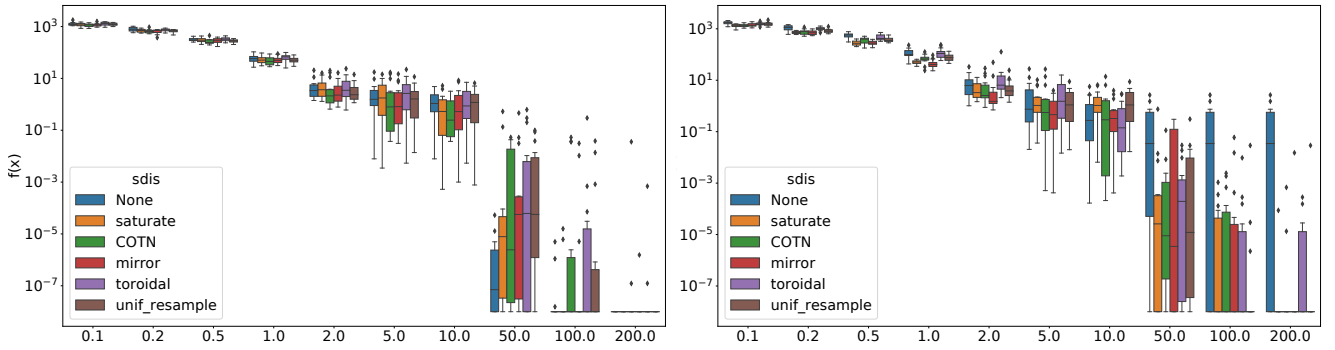
Figure 6: Performance of CMA-ES with center initialization on F13 of BBOB (left) and SBOX-COST (right) in 20D at various budgets (x-axis in thousands of function evaluations).
