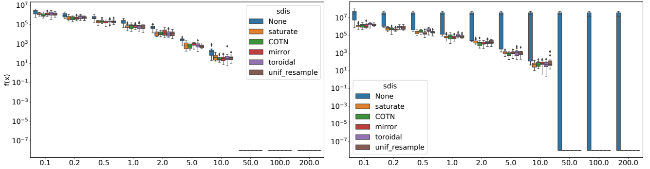
Figure 7: Performance of CMA-ES with uniform initialization on F2 of BBOB (left) and SBOX-COST (right) in 20D at various budgets (x-axis in thousands of function evaluations).
