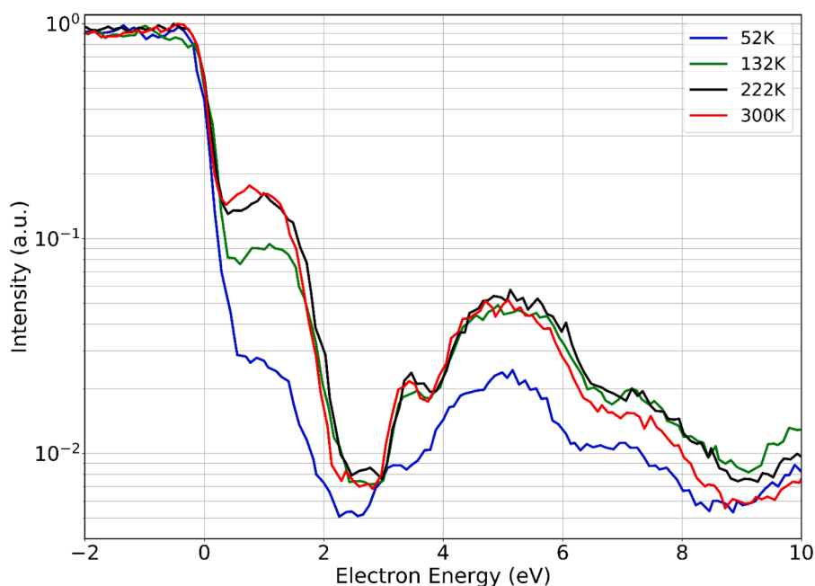
Fig. 6. LEEM-IV spectra of a three-monolayer pentacene film measured at different temperatures.
