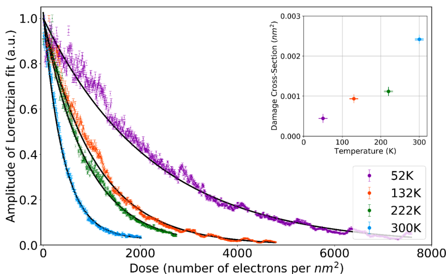
Fig. 5. Irradiation damage from a beam of 15 eV electrons to a pentacene film three monolayers in thickness. To quantify the damage, Lorentzian curves are fit to the spot profile of the 0th-order diffraction peak. The plot shows the decay of diffraction intensity over time, as a result of accumulated dose. Beam damage is obtained at four different temperatures of 52 K, 132 K, 222 K and 300 K. The solid black curves are simple exponential fits of the form Ae^{-\sigma \cdot D} + B , where D is the accumulated dose (horizontal axis), \sigma is damage cross-section in \text{nm}^2 , and A and B are constants. Cross-sections obtained from the fits are displayed in the inset figure. The colors correspond to the temperatures in the main figure legend.
