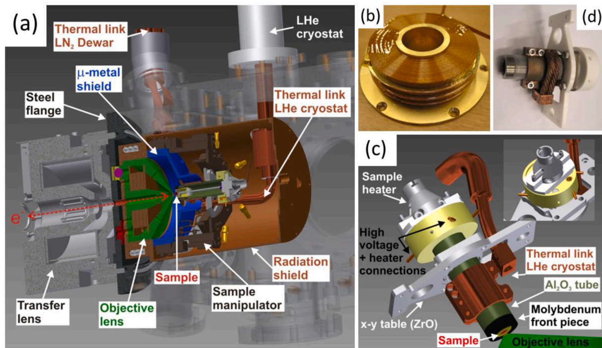
Fig. 2. Detailed schematic of the cryogenic sample chamber. (a) Schematic cross-section of the cryogenic setup. Electrons enter the chamber from the left. Various elements are highlighted and annotated. (b) Photograph showing the HTS coil assembly. The four disks are separated by 1-mm thick Au-plated copper plates (c) Schematic of the cryogenic sample holder, with its various components highlighted and annotated. The copper clamp around the sapphire tube is connected to the helium flow cryostat. (d) Photograph of the sample holder assembly.
