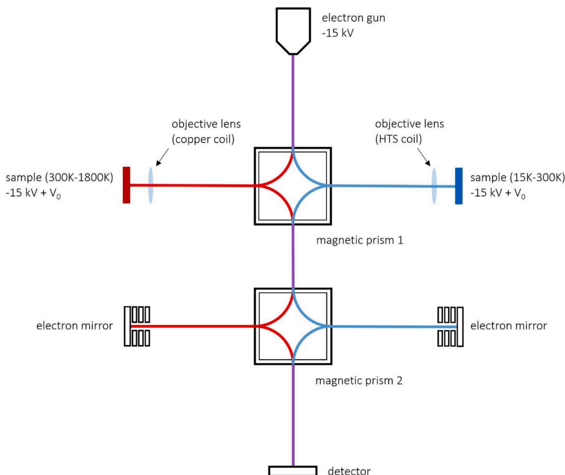
Fig. 1. Schematic of the ESCHER LEEM instrument. Electrons are emitted from the gun and go through the column with a kinetic energy of 15 keV. Before interaction with the sample, they are decelerated to a kinetic energy of eV_0 . The beam path for the cryogenic and room/high-temperature operation is indicated in blue and red, respectively. The central column is shared between the cryogenic and room-high-temperature sides (purple beam path). To maintain the required symmetry, the two sides have separate aberration-correcting electron mirrors. The objective lens coil for the room/high-temperature side is comprised of a copper coil, while for the cryogenic side, a high-temperature superconducting (HTS) coil is used to prevent Joule heating and, hence, reduce the total heat load.
