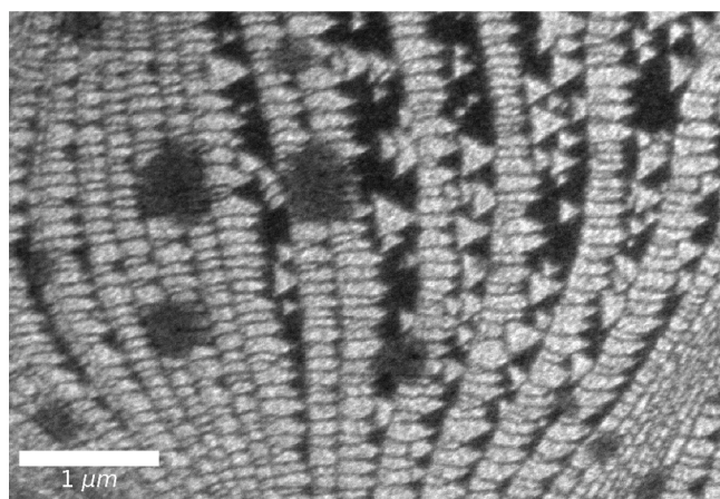
Fig. 4. Bright-field image of Si(111) 7 \times 7 surface reconstruction, imaged at 58 K with 10.3 eV electrons.
