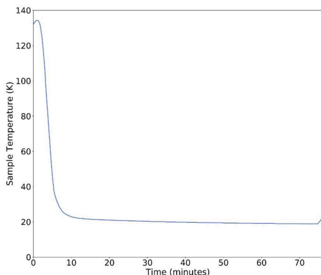
Fig. 3. Sample temperature during the final stage of sample cooling to 19 K. Note that the liquid He supply was stopped after 75 min.
