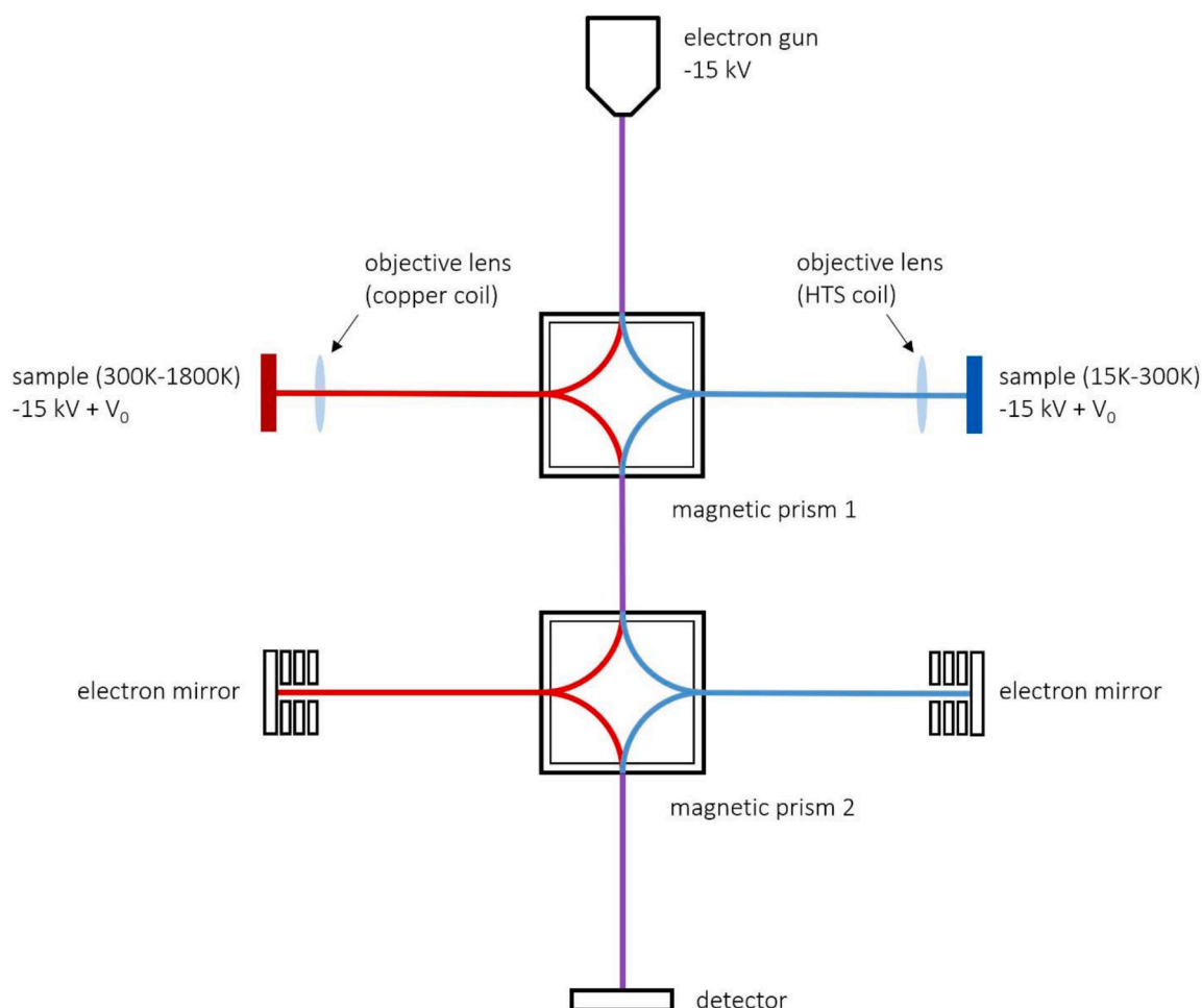
Fig. 1. Schematic of the ESCHER LEEM instrument. Electrons are emitted from the gun and go through the column with a kinetic energy of 15 keV. Before interaction with the sample, they are decelerated to a kinetic energy of eV_0 . The beam path for the cryogenic and room/high-temperature operation is indicated in blue and red, respectively. The central column is shared between the cryogenic and room-high-temperature sides (purple beam path). To maintain the required symmetry, the two sides have separate aberration-correcting electron mirrors. The objective lens coil for the room/high-temperature side is comprised of a copper coil, while for the cryogenic side, a high-temperature superconducting (HTS) coil is used to prevent Joule heating and, hence, reduce the total heat load.
