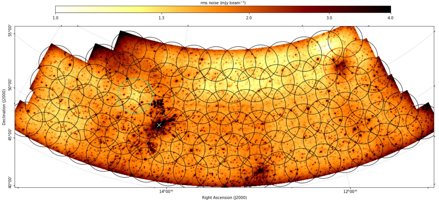
Fig. 11. Rms noise map of the LOFAR LBA Sky Survey - DR1. The regions with reduced sensitivity are located around bright sources that induce dynamic range limitations. Each pointing is shown with a circle at the FWHM. The red pointing (P174+57) was not observed, while the blue pointing (P218+55) was observed for 16 hrs (twice as much as the others). The white “x” indicates the position of the bright source 3C 295, which lowers the dynamic range in several fields around it.
