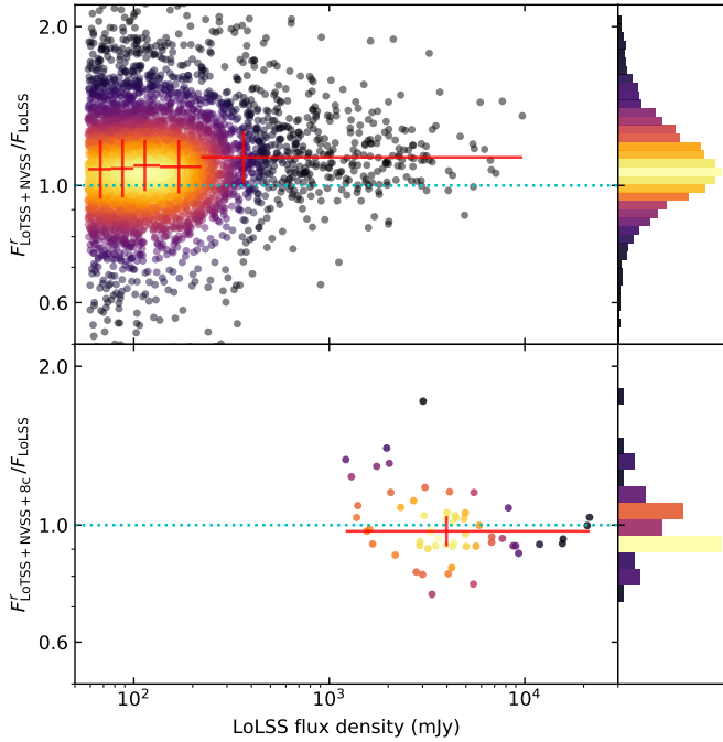
Fig. 15. LoLSS flux density versus the expected flux density at 54 MHz from the linear extrapolation of the spectral energy distribution (SED) using NVSS and LoTSS ( top panel ) or from a quadratic polynomial SED estimated using NVSS, LoTSS, and 8C ( bottom panel ). A ratio of 1, the blue dotted lines, means a perfect match between the prediction and the flux density measured in LoLSS. Red crosses are binned medians (five bins for the top panel , one for the bottom ) with \pm 1 median absolute deviation shown as an extension in the y -direction and the bin size as an extension in the x -direction.
