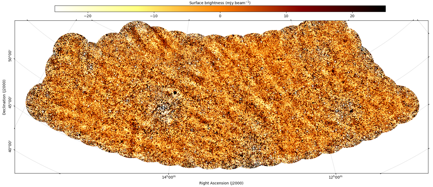
Fig. 7. Low-resolution (3'), source-subtracted map of the survey area. Large and locally aligned stripes of emission are visible crossing the region. The same structures were identified in the corresponding LoTSS images, which were calibrated independently with a different calibration code, demonstrating that these features are not artefacts.
