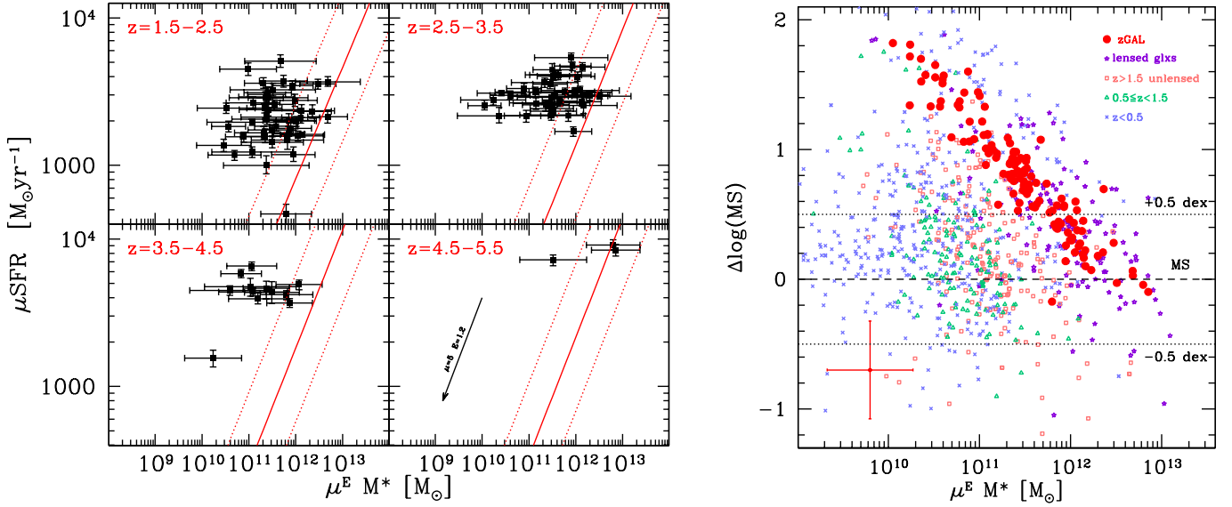
Fig. 12. Analysis of stellar masses, computed by inverting the \tau_{\text{dep}} scaling relation by Tacconi et al. (2020) as explained in Appendix A. Left panel: Position of the z-GAL (and pilot) sources in the SFR vs. M^* space. The red solid lines depict the MS of star-forming galaxies (Speagle et al. 2014) and the dotted lines mark the \pm 0.5 dex region around the MS. Both SFR and M^* are determined modulo the unknown magnification factor \mu . The arrow in the lower-right panel indicates the effect of applying a magnification correction with \mu = 5 and E = 1.2 . Right panel: Distance from the MS, \Delta\log(\text{MS}) = \log(\mu\text{SFR}/\text{sSFR}(\text{MS}, z, M^*)) , as a function of stellar mass, M^* . The dotted horizontal lines represent the range \pm 0.5 dex from the MS (dashed line). The position of z-GAL galaxies is marked with filled circles and literature data are as in Fig. 10. The median uncertainty of the quantities derived for z-GAL galaxies is shown in the bottom left. See Sect. 6 and Appendix A for more details.
