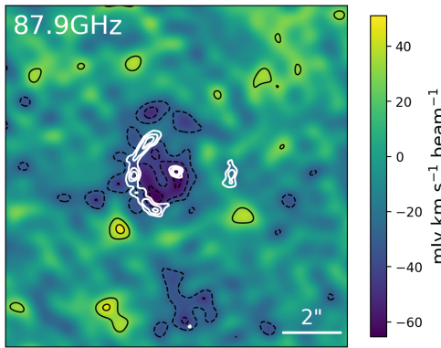
Fig. A.1. Image of the absorption feature at 87.9 GHz, made from the continuum-subtracted data using a 250-k \lambda uv-distance cut. The black contours start at \pm 2\sigma and increase in steps of 1\sigma , white contours indicate the Band 3 continuum. The absorption is not associated with the lensing arcs and is most likely due to a foreground CO(0–1) absorber at z \approx 0.31 .
