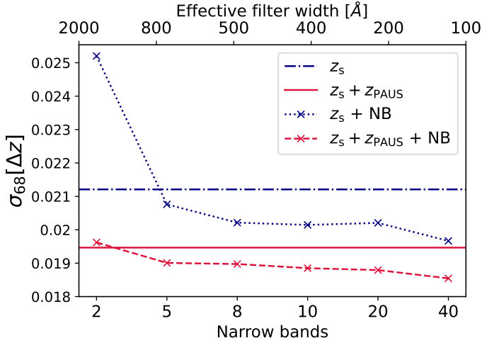
Fig. 14. Photo- z precision as a function of number of bands in the predicted photometry for z_s + NB (dotted blue line) and z_s + z_{PAUS} + NB (dashed red line). The horizontal line corresponds to the z_s (dashed-dotted blue line) and z_s + z_{PAUS} (solid red line), where MTL is not enabled.
