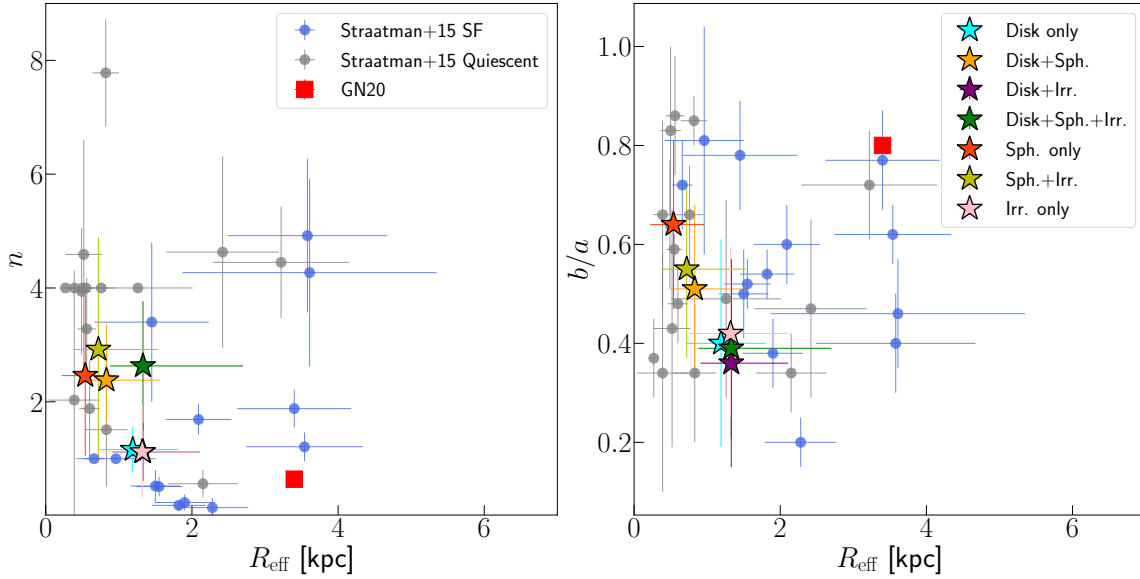
Fig. 4. Structural parameters, R_{\text{eff}} - n (left) and R_{\text{eff}} - b/a (right), for different populations of z \sim 4 galaxies. Blue and grey circles represent the massive star-forming and quiescent galaxies, respectively, from the ZFOURGE and CANDELS surveys (Table 1 of Straatman et al. 2015 ). Coloured stars display the mean values for each one of the morphologically-classified groups of CEERS galaxies (Table 1 of Kartaltepe et al. 2023 ). The red squares are the values for GN20 and their sizes include their associated errors.
