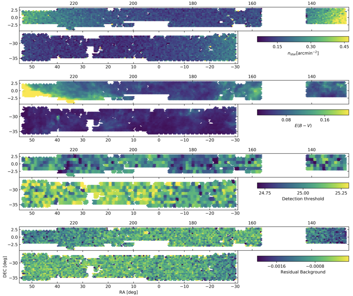
Fig. 8. HEALPIX maps of the density of Gaia DR2 stars with 14 < G < 17 in the KiDS DR4 footprint ( first row ), galactic dust extinction ( second row ), detection threshold above background ( third row ), and residual background ( fourth row ). All maps were generated with n_{\text{side}} = 256 .
