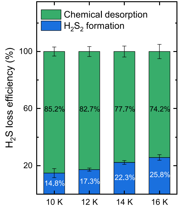
Fig. 6. Derived contributions from \text{H}_2\text{S}_2 formation and \text{H}_2\text{S} chemical desorption to the measured loss in N(\text{H}_2\text{S}) after 120 min of H-atom exposure at 10, 12, 14, and 16 K.
