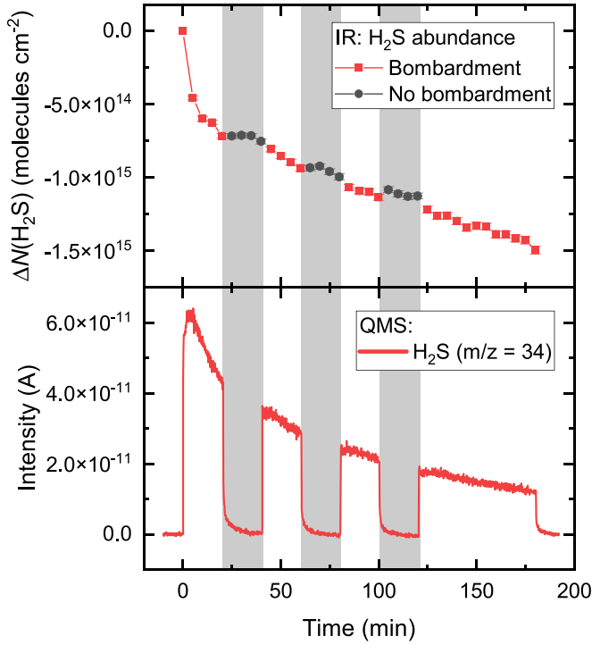
Fig. 5. Monitoring of \text{H}_2\text{S} in the solid and gas phases during H-atom bombardment. Upper panel: variation in \text{H}_2\text{S} column density measured from the \sim 2553\text{ cm}^{-1} band in the IR spectra as a function of time. Lower panel: scan of the m/z = 34 ( [\text{H}_2\text{S}]^+ ) as measured by the QMS as a function of time. The shadowed areas denote the periods during which the H-atom flux was stopped.
