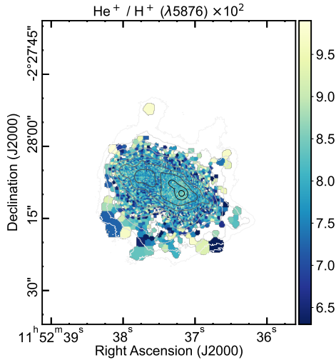
Fig. 9. Map for the \text{He}^+/\text{H}^+ abundance derived from the \text{He I } \lambda 5876 emission line. North is up and east towards the left.
