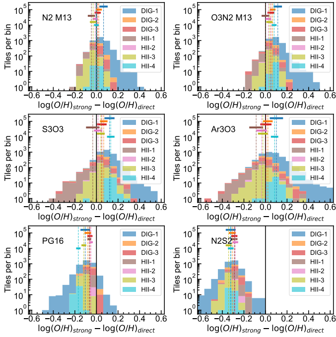
Fig. 23. Histograms with the difference between the oxygen abundance, 12 + \log(\text{O}/\text{H}) , as derived from different strong line methods and the direct method, in the different regions defined with astrodendro . Vertical dashed lines denote the mean of a given distribution while the length of thick horizontal bands is the standard deviation. The order of the rows and columns is the same as in Fig. 22.
