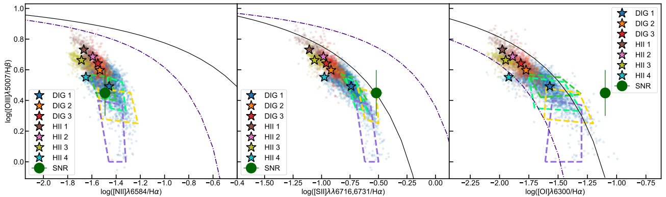
Fig. 13. Position of the individual tiles (small translucent stars) and the regions defined by astro dendro (large solid stars) in the so called BPT diagnostic diagrams (Baldwin et al. 1981). Black continuous lines show the theoretical borders proposed by Kewley et al. (2001) to delimit the area where the line ratios can be explained by star formation, while indigo dashed-dotted lines mark the maximal starburst prediction for an object with metallicities Z = 0.004 , as derived by Xiao et al. (2018). The big green circle in each diagram represents the line ratios for the unresolved source at RA (J2000) = 11:52:37.8 and Dec (J2000) = -02:28:03.0 , once fluxes have been decontaminated by the diffuse gas emission of the galaxy. The four irregular polygons with dashed lines approximately delimit the loci of line ratios measured in the regions marked in Fig. 3.
