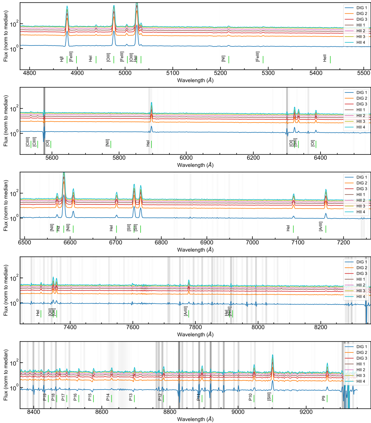
Fig. 4. Integrated spectra for the regions defined by astrodendro . Fluxes are presented in logarithmic stretch to optimally visualise at the same time bright and faint features. Spectra have been offset by a factor \times(1 + 2N) with N the spectrum number, as indicated by the alphabetically ordering of the labels, to avoid an overlap of the spectra. Small vertical limegreen lines indicate the expected position of the relevant emission lines. The vertical grey bands mark the position of the brightest skylines, the stronger the line is, the more opaque the band appears.
