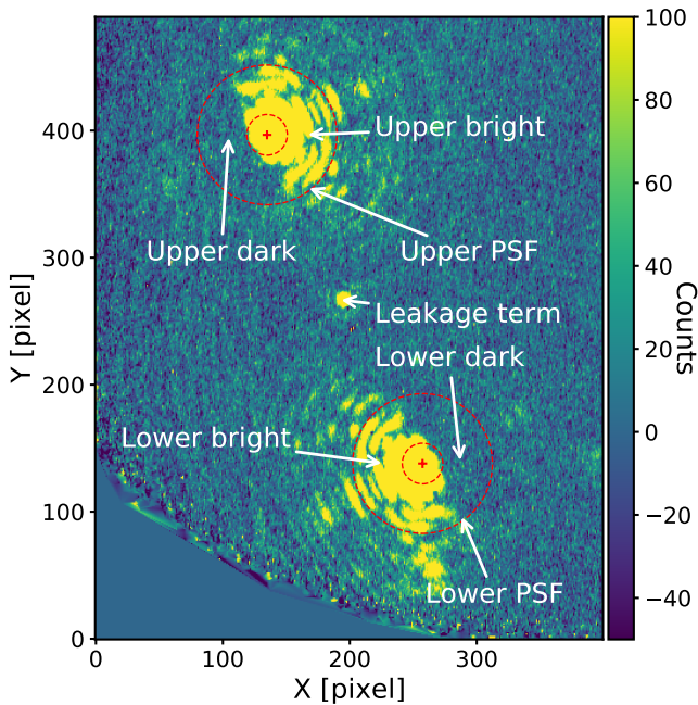
Fig. 2. On-sky coronagraphic PSF from the gvAPP180 mounted on MagAO/Clio2 at 3.94 \mu m. One PSF (upper PSF) is above another PSF (lower PSF) with a leakage term in the middle. The red circles in dashed lines show the IWA and OWA. The dark holes of the two PSFs complement the FoV of each other. The four different regions of the two PSFs we defined in this work are marked with white text. The colourbar shows the flux intensity after background subtraction.
