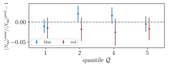
Fig. B.3. Mean aperture number of the red and blue sample, where the predictions follow from a joint minimisation process. Different to the full bright sample the measured p(N_{ap}) is smaller than the predicted Map, resulting in the measured \langle N_{ap} \rangle being smaller.
