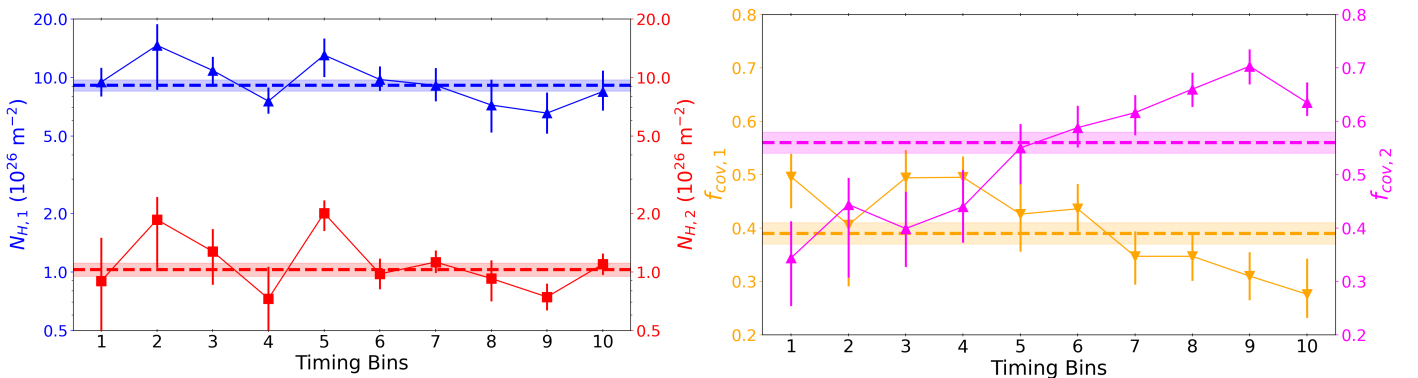
Fig. A.1. Comparing the parameters of the two obscurer model; details are discussed in Appendix A. Left: Column densities of the two obscurer components, blue for obscurer component 1 ( N_{\text{H},1} ) and red for component 2 ( N_{\text{H},2} ). Right: Covering fractions of the two obscurer components, orange for obscurer 1 ( f_{\text{cov},1} ) and magenta for obscurer 2 ( f_{\text{cov},2} ). The dashed lines in each panel show the time-averaged best fit parameter values, with their uncertainties displayed as the shaded areas.
