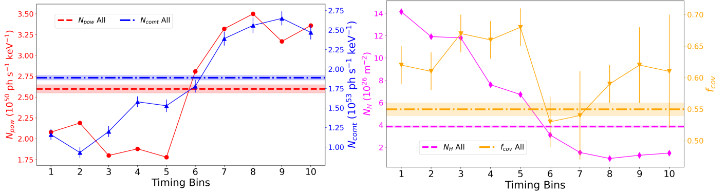
Fig. 11. Further tests to determine the cause of the observed variability. Left: Fixing the obscurer parameters to their time-averaged values in Obs 1 (Table 3), and fitting N_{\text{pov}} (red circles) and N_{\text{comt}} (blue triangles) in each TB. Right: Fixing the continuum parameters to their time-averaged values and fitting N_{\text{H}} (magenta diamonds) and f_{\text{cov}} (orange triangles). In both scenarios the changes in the parameters suggest that they could contribute to the observed variability. See Sect. 5.3 for details. The uncertainties on N_{\text{pov}} (left) and N_{\text{H}} (right) are relatively small that they are within the data points. The photon index and reflection scaling parameters from the continuum show the same trends as Fig. 7 when the obscurer parameters are fixed. The ionisation parameter of the obscurer does not change when the continuum parameters are fixed.
