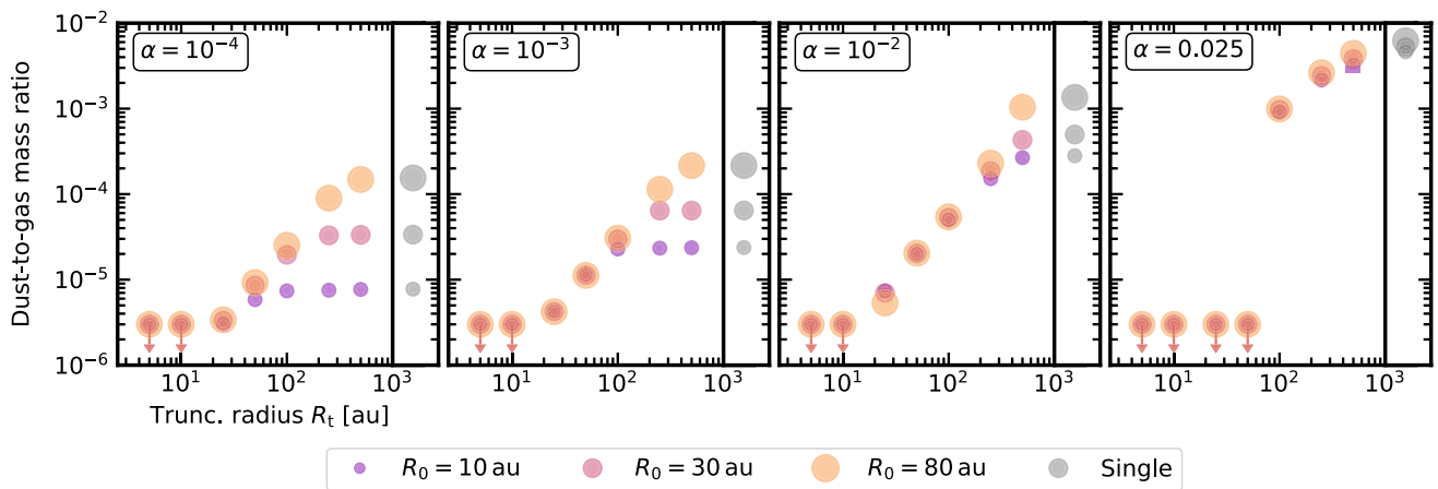
Fig. 1 The dust-to-gas mass ratio in circumstellar binary discs increases with the companion separation (2 Myr snapshot). Single discs are in grey, while different colours/sizes display different values of R_0
