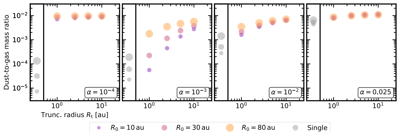
Fig. 3 The dust-to-gas mass ratio in circumbinary discs substantially depends on viscosity and only moderately increases with binary separation (2 Myr snapshot). Single discs are in grey, while different colours/sizes display different values of R_0
