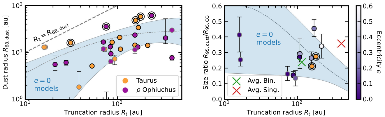
Fig. 2 Left: Disc dust sizes in Taurus (orange) and \rho Ophiuchus (purple) binary discs as a function of the truncation radius. The measured sizes are compatible with e = 0 models (shaded blue region). An outer ring identifies the substructured discs, and black/grey marker edges identify primary/secondary discs. Right: Dust-to-gas size ratio as a function of the truncation radius in Taurus. The data points, colour-coded by eccentricity (orange if e is not known), are compatible with e = 0 models (shaded blue region). Green and red crosses show the average dust-to-gas size ratios in binaries (plotted at the average truncation radius) and singles (plotted at an arbitrary large radius)
