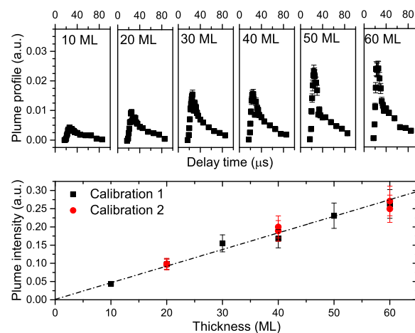
Fig. 1. Calibration measurements for LDPI TOF MS of \text{H}_2\text{O} ice. Top panel: LDPI TOF MS plume profiles for different initial \text{H}_2\text{O} ice thickness at 20 K. The intensity is the sum of the m/z = 17 ( \text{OH}^+ ) and m/z = 18 ( \text{H}_2\text{O}^+ ) signals, which are the two major fragment masses upon electron impact ionization of water. Profiles were collected as a function of the delay time between laser desorption and ion extraction. Bottom panel: total signal of the integrated plume profiles from the top panel as a function of initial ice thickness of amorphous \text{H}_2\text{O} ice, collected during two independent calibration measurements. The data were fitted with a linear function ( R^2 = 0.98 ).
