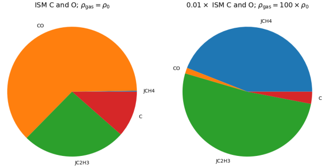
Fig. B.3: Most abundant species in the model presented in figure 4(a), (left panel) and the model presented in figure B.1(d), (right panel) for a disk age of 5 Myr. Molecules with a ‘J’ denote species that are frozen onto dust grains. The abundances are integrated between 50 AU and 70 AU (i.e. near the millimeter dust ring) and from the midplane to z/r = 0.43 . It therefore includes the main reservoir of CO that contributes to the C^{18}O flux. It is clear that when the abundances of carbon and oxygen are reduced, the main reservoir of carbon is shifted towards hydrocarbons that are frozen onto the dust.
