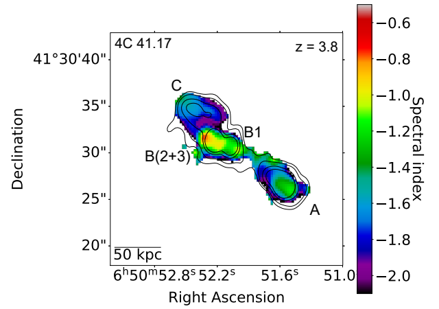
Fig. 2. Map of the low-frequency 144 MHz – 1.4 GHz spectral index of the Anthill at z = 3.8 obtained using the ILT HBA and VLA L -band observations. The ILT HBA contours from the smoothed 144 MHz image in Fig. 1 are also displayed on the spectral index map.
