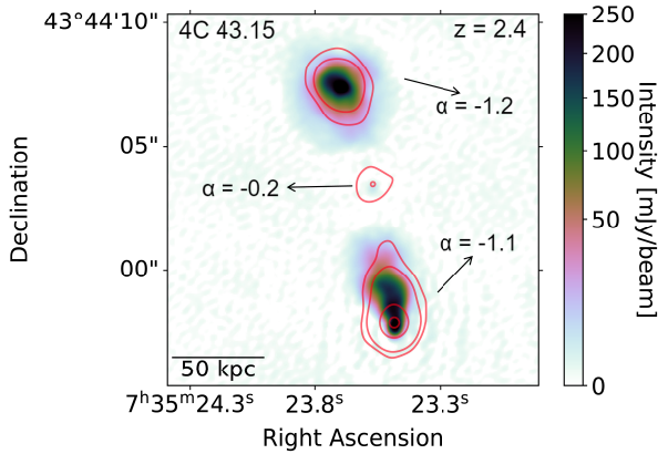
Fig. 9. ILT 144 MHz final processed image of 4C 43.15 at z = 2.4 , with a resolution of 4'' \times 4'' and the VLA contours in X band.
