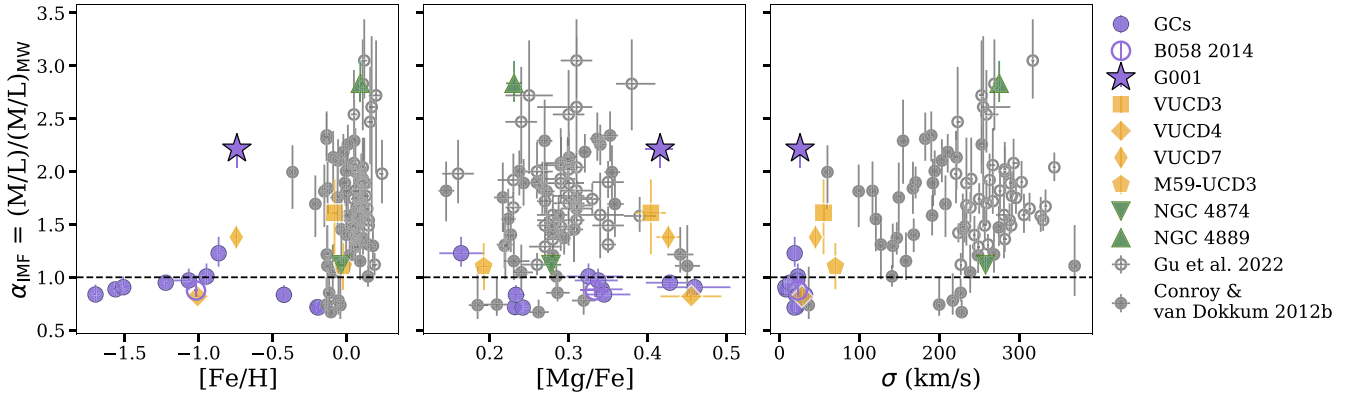
Figure 9. The IMF mismatch parameter, \alpha_{\text{IMF}} , as a function of stellar parameters, including fitted [Fe/H] (left), fitted [Mg/Fe] (middle), and literature velocity dispersion ( \sigma , right). This is similar to figure 3 in V17. The GCs are shown as large, filled circles. G001 (star) is highlighted to show its deviation from the main body of GC results. The newly reduced B058 data from V17 (open symbol) is highlighted to demonstrate the consistency between data taken on different dates and reduced differently. The UCDs are shown as separate symbols and the BCGs are shown as triangles. We also include the sample of ETG values from Conroy & van Dokkum (2012b) (data refitted here) as small, filled circles and from Gu et al. (2022) as small, open circles. The dashed line represents the value of \alpha_{\text{IMF}} for a Kroupa IMF.
