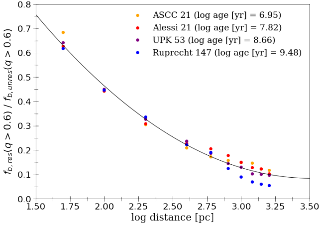
Fig. 7. Ratio of the fraction of resolved binaries over the fraction of unresolved binaries, both of systems with q > 0.6 ( \frac{f_{b,res}^{sim}(q > q_{lim}=0.6; d)}{f_{b,unres}^{sim}(q > q_{lim}=0.6; d)} ), as a function of logarithmic distance, for four open clusters simulated with GOG. The black solid curve is the quadratic fit to the four open clusters that we use to compute the total multiplicity fraction.
