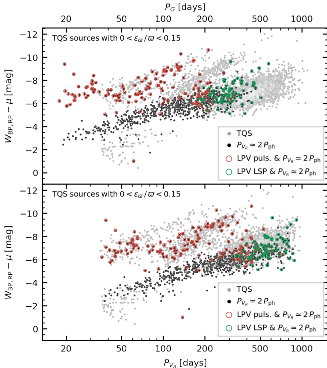
Fig. 32. Similar to the right-hand side panels in Fig. 30, but with the sources having P_{VR} \approx 2P_{ph} highlighted in black. The PLD constructed with P_G is shown in the top panel and the one constructed with P_{VR} in the bottom panel for the TQS sources with parallax errors better than 15% (gray symbols), and highlighting the sources with P_{VR} \approx 2P_{ph} . Red and green circles indicate LPVs showing pulsation and a LSP, respectively. Only five of them are identified as C-rich.
