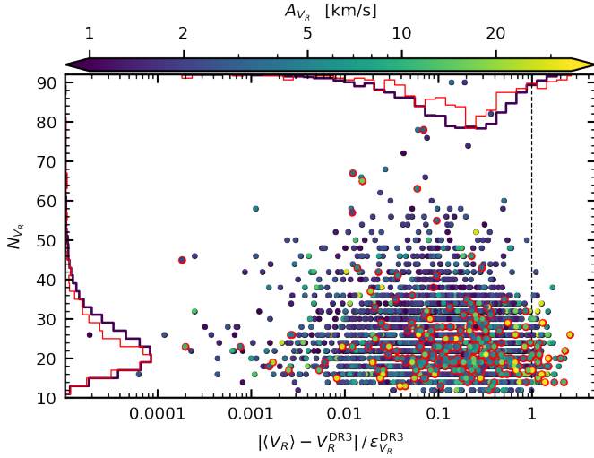
Fig. 15. Number N_{VR} of epochs retained for RV variability processing against the absolute difference between the median RV derived by variability processing ( \langle V_R \rangle ) and published in Gaia DR3 ( V_R^{DR3} ), scaled to the RV uncertainty \epsilon_{VR} published in DR3. Data points are color-coded by the semi-amplitude of the RV time series model. The time series that had one RV epoch excluded by outlier removal during variability processing are circled in red. The value \langle V_R \rangle for these sources is computed from one fewer epoch compared to V_R^{DR3} .
