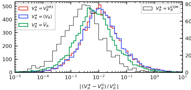
Fig. 16. Comparison of several average RV indicators with the zero point of the RV time series models. Different indicators are displayed in different colors (red: median value V_R^{DR3} published in Gaia DR3; blue: median value \langle V_R \rangle computed by variability processing; green: mean value \bar{V}_R computed by variability processing). The histograms show the distribution of absolute difference between each of the average values and V_R^0 , normalized to the latter. The thin black histogram, limited to a subset of the FPR sample, compares V_R^0 with the center-of-mass velocity V_R^{COM} derived by the non-single stars processing pipeline for Gaia DR3 (see Sect. 4.1.2 for more details), and refers to the scale on the right-hand side axis.
