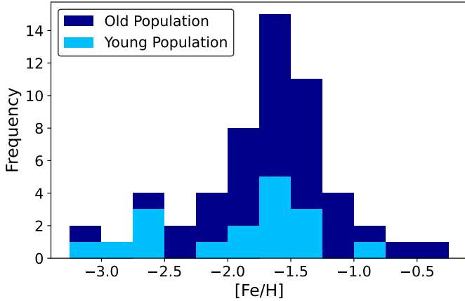
Fig. 5. Distribution of the metallicity ( [Fe/H] ) of 55 Leo T stars estimated using spexxy . The younger population, consisting of 17 stars, is represented with a lighter colour.
