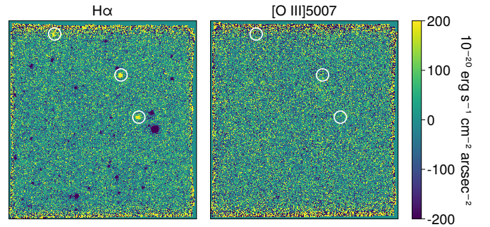
Fig. 14. Narrow-band images over \text{H}\alpha (left) and \text{O}[\text{III}]\text{5007} (right). In the left-hand panel the three emission line stars are easily seen, but no evidence is found of extended emission in either \text{H}\alpha or \text{O}[\text{III}]\text{5007} .
