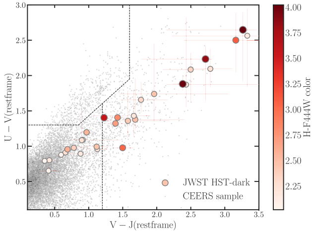
Figure 4. UV against VJ rest-frame colours diagram. HST -dark galaxies are presented as big circles with the H\text{-F444W} color on the third axis, whereas the grey dots are the total CEERS sample. The black-dashed lines show the usual classification of galaxies in quiescent, star-forming and dusty from Spitler et al. (2014). Our sample of HST -dark galaxies lies mostly in the dusty colour space with part of the sample in the star-forming galaxy region. There are no quiescent galaxies in our selection due to the colour cut; however, given the photometric uncertainties, we cannot exclude that some of the galaxies are quiescent.
