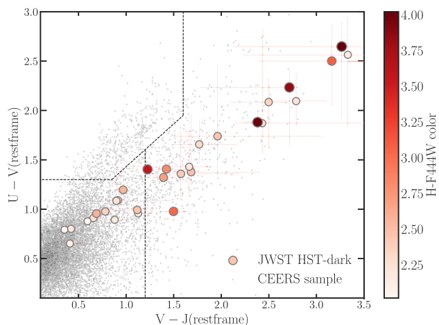
Figure 4. UV against VJ rest-frame colours diagram. HST -dark galaxies are presented as big circles with the H\text{-}F444W colour on the third axis, whereas the grey dots are the total CEERS sample. The black-dashed lines show the usual classification of galaxies in quiescent, star-forming and dusty from Spitzer et al. (2014). Our sample of HST -dark galaxies lies mostly in the dusty colour space with part of the sample in the star-forming galaxy region. There are no quiescent galaxies in our selection due to the colour cut; however, given the photometric uncertainties, we cannot exclude that some of the galaxies are quiescent.
