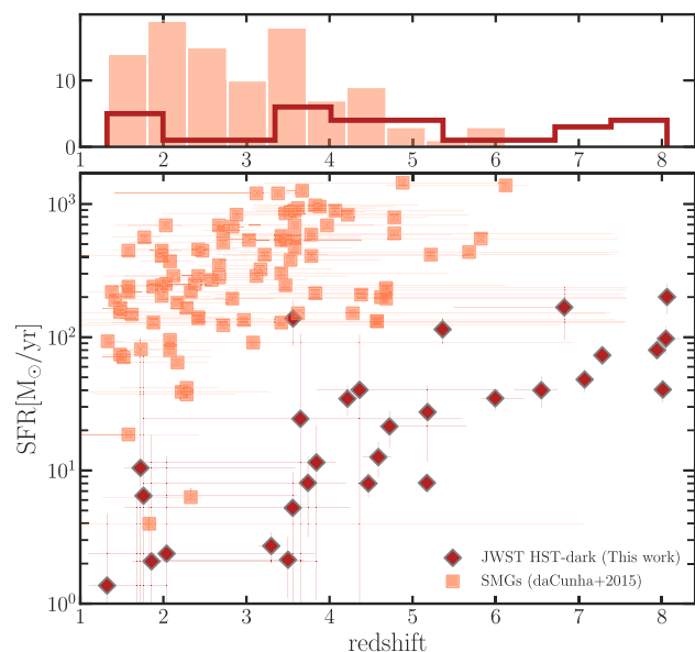
Figure 5. HST -dark galaxies compared with SMGs. Top panel: The redshift histogram shows that HST -dark galaxies (red line) lie mostly at z > 3.2 and extend to higher redshift compared to SMGs (orange bars). Bottom panel: Photometric redshifts against SFRs. On average, HST -dark galaxies lie at higher redshift and have significantly lower SFRs [orange squares; ALESS sample from da Cunha et al. (2015)]. The significantly smaller error bars in the photometric redshifts are due to the improvement coming from the deep, high-resolution JWST /NIRCam data.
