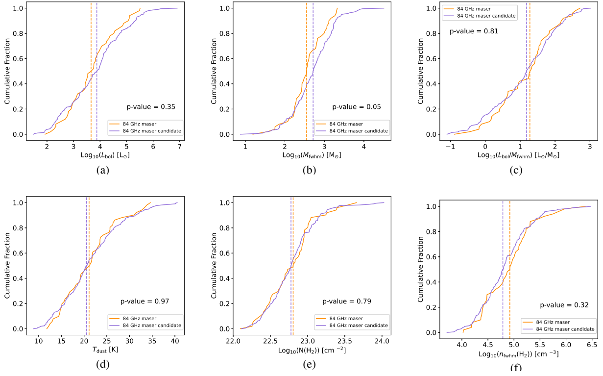
Fig. B.3. Cumulative distribution functions of the physical properties for the clumps with 84 GHz methanol masers and maser candidates. In panels (a) to (f) are plotted the cumulative distributions of the bolometric luminosity, the FWHM clump mass, the luminosity-to-mass ratio, the dust temperature, the peak \text{H}_2 column density, and the mean \text{H}_2 FWHM volume density for 84 GHz methanol masers (orange lines) and maser candidates (purple lines), respectively. The vertical dashed lines in the corresponding colours depict the median values of the two samples. The p-values from the K-S tests are presented in each panel.
