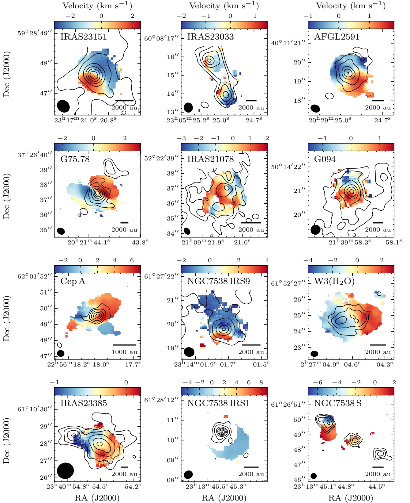
Fig. E.2: Maps of offset velocity with respect to the systemic velocity obtained by fitting CH 3 CN(12 K - 11 K ) K = 0 - 6 and CH 3 13 CN(12 K - 11 K ) K = 0 - 3 lines with XCLASS for the best disk candidates in the CORE survey. The contours correspond to the 1.37 mm continuum as described in Fig. 1. For NGC7538 IRS1, only the region outside the continuum to the south-west is modelled by XCLASS as the molecular lines are seen in absorption against the strong continuum source with many velocity components due to the complex dynamics in this source. The synthesised beam is shown in the bottom left corner and a scale bar in the bottom right corner of each panel.
