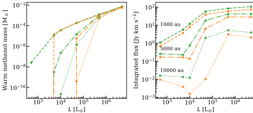
Figure 8.13: Warm methanol mass (left) and integrated line flux of methanol (right) for envelope-only fiducial models with different luminosities and carved HC or UC HII regions. Green and orange show low and high mm opacity dust models. Dashed lines show when the size of HII region is 1000 au, dashed dotted lines show the same for 5000 au, and the dotted lines show the same for 10000 au. An HII region of size \sim 10000 au is needed for a drop of \gtrsim 2 orders of magnitude in methanol emission.
