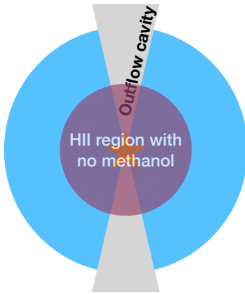
Figure 8.12: Sketch of the potential HC or UC HII region around a high-mass protostar. It is expected that methanol is absent in this region as the gas is atomic and ionized.
