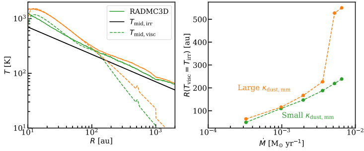
Figure 8.3: Comparison of the midplane temperature calculated by RADMC-3D for the fiducial envelope-plus-disk model (left; solid orange and green lines), and the same calculated from viscous heating analytically (dashed lines) and found from passive heating from the protostar analytically (solid black line). Green shows dust with small \kappa_{mm} , and orange shows dust with large \kappa_{mm} . Radius at which the analytical midplane temperature from viscous heating equals that from passive heating, plotted against the mass accretion rate for the fiducial model and for the model with high mm opacity dust (right).
