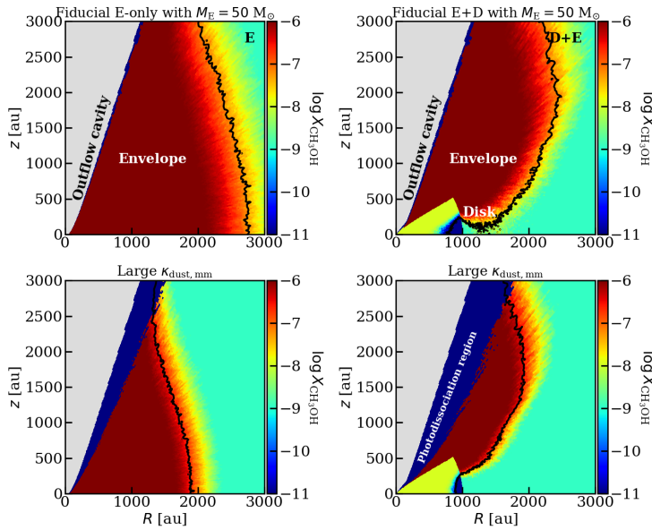
Figure 8.B.4: Same as Fig. 8.7, but now for M_E = 50 M_\odot . The photodissociation regions for the models with high mm opacity dust are significant.
