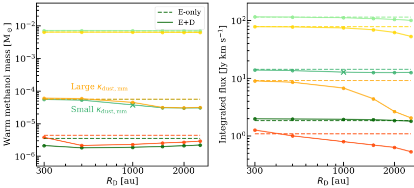
Figure 8.10: Warm methanol mass (left column) and integrated methanol emission (right column) for various disk sizes. The various shades of green and orange are used to indicate variations in luminosity. The luminosity from low to high is indicated by the darkest to lightest color. The models plotted here have luminosities 5 \times 10^2 L_\odot , 1 \times 10^4 L_\odot and 5 \times 10^6 L_\odot . The dashed lines present fiducial envelope-only models with various luminosities. The solid lines present the fiducial envelope-plus-disk models with various luminosities and disk radii. The shades of orange show models with large dust grains (high mm opacity), and the shades of green show those with small grains (low mm opacity).
