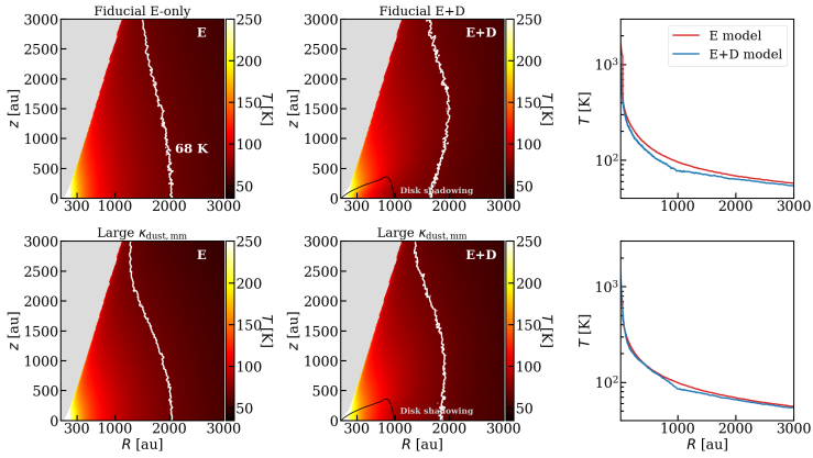
Figure 8.2: Temperature structure of the fiducial envelope-only and envelope-plus-disk. The top row shows the models with low mm opacity dust ( \kappa_{1\text{ mm}} \simeq 0.2\text{ cm}^2\text{ g}^{-1} ), and the bottom row shows models with high mm opacity dust ( \kappa_{1\text{ mm}} \simeq 18\text{ cm}^2\text{ g}^{-1} ). The right column shows a temperature cut for the various models at z = 0\text{ au} . The white contours show where the temperature is 68 K (roughly where methanol sublimates from the grains). The black contours show the approximate position of the disk.
