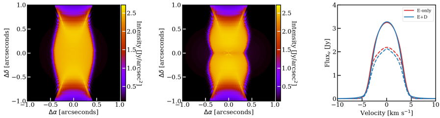
Figure 8.B.2: Methanol emission from the fiducial envelope-only and envelope-plus-disk models. The left and middle panels show the emission at the peak of the line viewed edge-on for the two models without dust in these two particular models, so that the methanol emission can be seen without optical depth effects from the dust (dust is included in all other models, unless otherwise stated). The right panel shows the continuum-subtracted line flux at an assumed source distance of 4 kpc when viewed edge-on (solid lines) and face-on (dashed lines).
