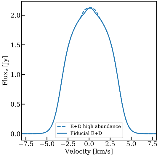
Figure 8.B.9: Methanol line emission for the fiducial envelope-plus-disk model (solid line) and the same with disk abundances that are two orders of magnitude higher (dashed line).
