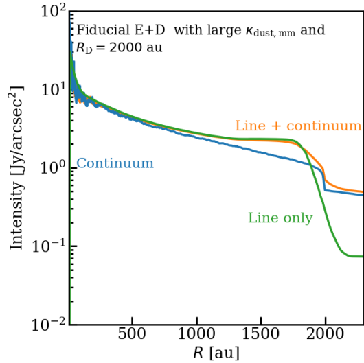
Figure 8.B.7: Intensity cut through the fiducial model with high mm opacity dust and a disk radius of 2000 au. Orange shows the model when dust and gas are included in the run, blue shows the model when only dust is included, and green shows the model without dust. The intensity of the line, the continuum, and the continuum plus line in the inner \sim 1500 au are similar while continuum subtraction will result in almost zero intensities.
