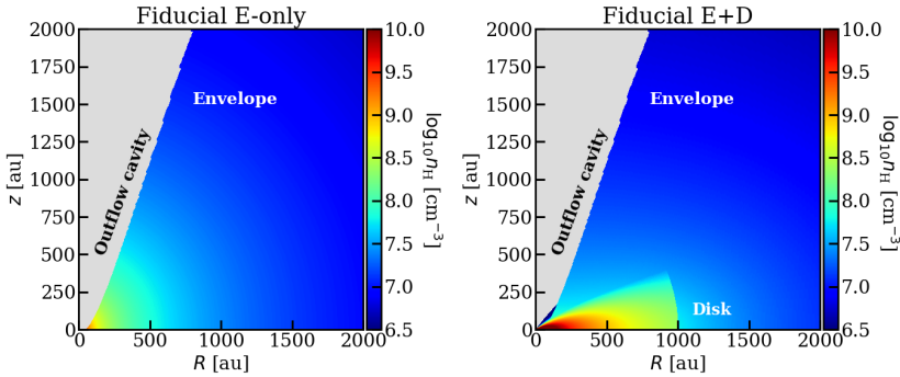
Figure 8.1: Gas density profiles. Two-dimensional total hydrogen nucleus number density for the fiducial envelope-only model (left). The same, but for the fiducial envelope-plus-disk model (right). The outflow cavities in this and subsequent figures are masked gray.
