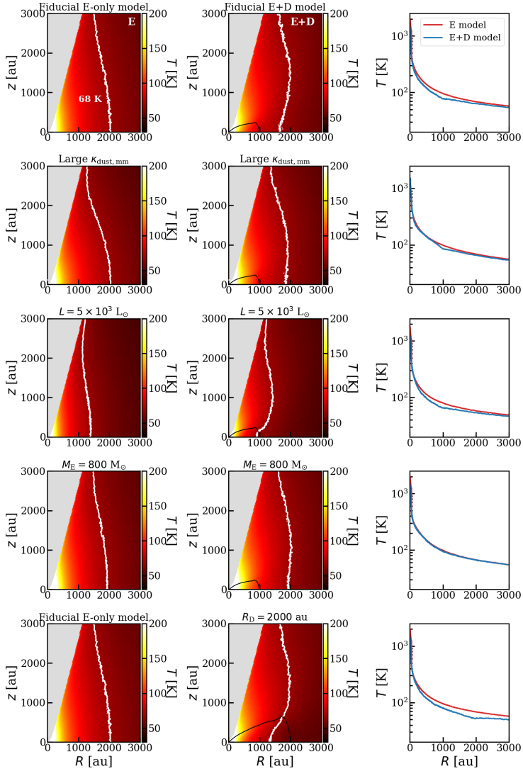
Figure 8.B.6: Temperature structure of models with different parameters. The left column presents the envelope-only models, the middle column shows the envelope-plus-disk models, and the right column presents the comparison of a temperature cut at z = 0 au between the two models. The rows from top to bottom show the fiducial model, the model with high mm opacity dust, with a protostellar luminosity of 5 \times 10^3 L_{\odot} , with an envelope mass of 800 M_{\odot} , and finally, the fiducial model with a disk radius of 2000 au.
