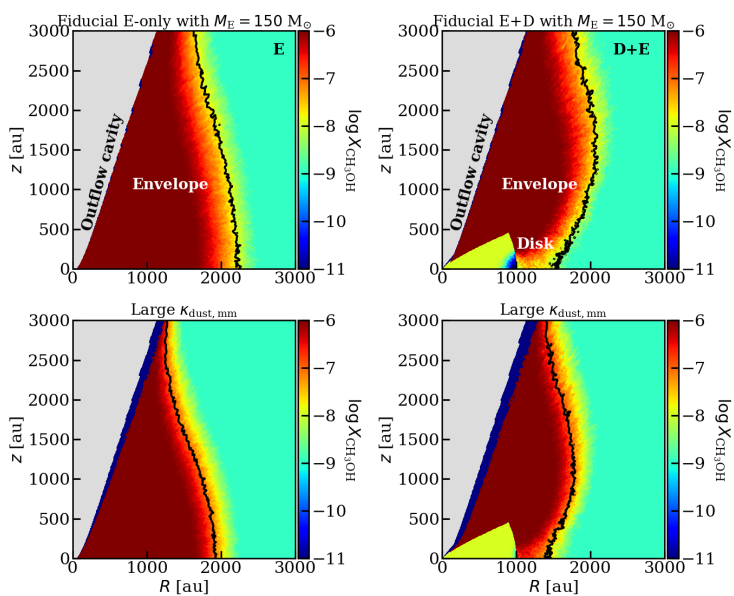
Figure 8.B.5: Same as Fig. 8.7, but now for M_E = 150 M_\odot .
