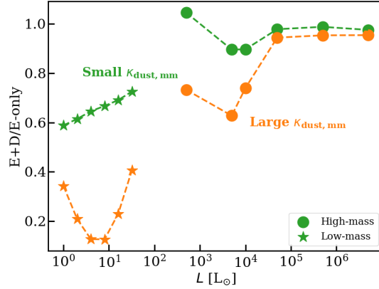
Figure 8.9: Comparison of methanol integrated fluxes between low- and high-mass protostars. The values for low-mass protostars are taken from Nazari et al. (2022b). The circles show the ratio of methanol-integrated fluxes of fiducial envelope-plus-disk models with varying luminosity to those of envelope-only models for high-mass protostars. The stars show the same for low-mass protostars. Green shows low mm opacity dust, and orange shows high mm opacity dust. Low-mass disks are more effective in decreasing the methanol emission than high-mass disks.
