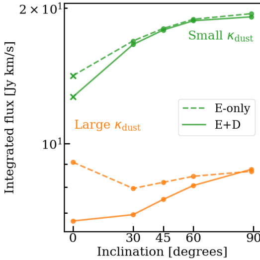
Figure 8.B.3: Integrated methanol flux as a function of viewing angle for the fiducial envelope-only and envelope-plus-disk models and for models with high mm opacity dust. The difference in integrated flux is smaller than a factor of 2 when the viewing angle changes.
