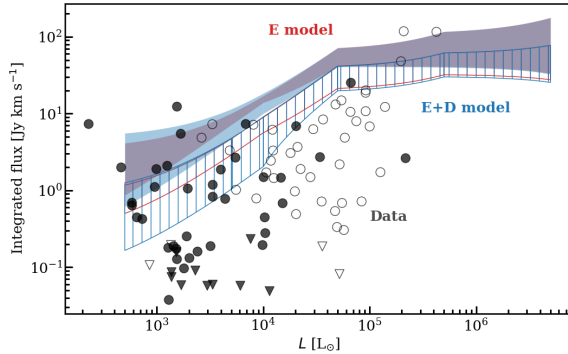
Figure 8.11: Comparison of models with observations of ALMAGAL sources. The same methanol line is used for the models and observations. Moreover, the integrated fluxes from the observations are normalized to a distance of 4 kpc to match those from the models. The black data points present the observations, where the circles are detections and triangles are upper limits. The empty symbols indicate sources whose L/M from Elia et al. (2017) is above 22.4 L_{\odot} M_{\odot}^{-1} , proposed to be ‘HII region candidates’. The smooth red and blue regions show the results from the envelope-only and envelope-plus-disk models with low mm opacity dust grains. The striped regions show the same for models with high mm opacity dust. The regions into which the models fall (blue and red) are found by simply connecting the integrated fluxes at the six different luminosities considered in this work in linear space.
