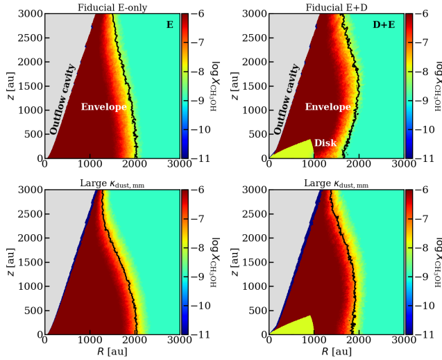
Figure 8.7: Gas-phase methanol abundance map for the fiducial envelope-only and envelope-plus-disk models (top row) and those with high mm opacity dust (bottom row). The black contours show the 68 K lines at which methanol starts to be sublimated from the grains at the densities of these models.
