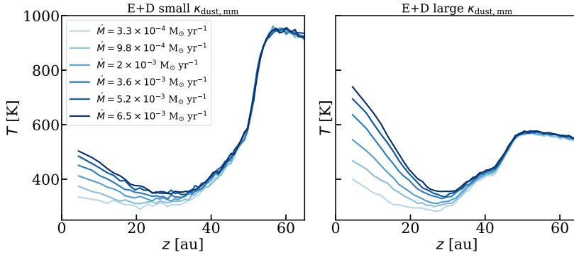
Figure 8.4: Vertical temperature cut at a radius of \sim 50 au. Left: Fiducial envelope-plus-disk model with varying envelope masses and thus various mass accretion rates. Right: Same as in the left panel, but for the fiducial models with large \kappa_{\text{dust, mm}} . The z of \sim 50 - 60 au marks approximately where the outflow cavity wall and hence the highest z at the disk or envelope surface at a radius of \sim 50 au is reached.
