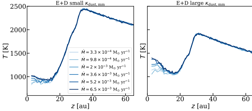
Figure 8.B.1: Same as Fig. 8.4, but when the bolometric luminosity is 5 \times 10^5 L_{\odot} and the vertical temperature cut is made at 30 au.
