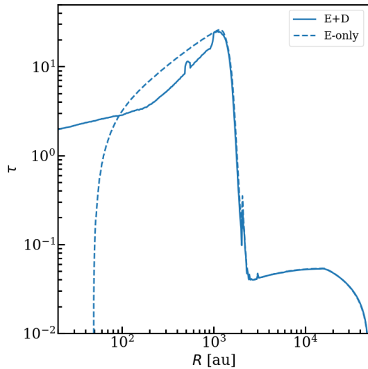
Figure 8.B.8: Methanol optical depth as a function of radius at the peak of the line. The dashed and solid lines show the fiducial envelope-only and envelope-plus-disk models, respectively. The emission is optically thick inside the snow surface.
