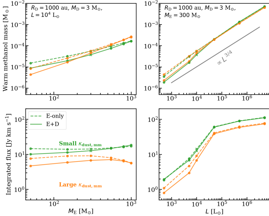
Figure 8.8: Warm methanol mass (top row) and integrated line fluxes (bottom row) for various models. The left column presents the models with varying envelope masses but constant luminosity of 10^4 L_{\odot} (i.e., varying accretion rates for the envelope-plus-disk models). The right column shows the models with varying bolometric luminosity but constant envelope mass of 300 M_{\odot} (i.e., constant accretion rate of 2 \times 10^{-3} M_{\odot} \text{ yr}^{-1} ). The parameters that were fixed for each column are printed in the top row plots. For example, where the envelope mass was varied, the disk radius was fixed to 1000 au, the disk mass was fixed to 3 M_{\odot} , and the luminosity was fixed to 10^4 L_{\odot} . Orange and green show the models with high and low mm opacity dust. The fiducial models are indicated by a cross. Solid and dashed lines present the envelope-plus-disk and envelope-only models, respectively. The solid gray line in the top right panel shows the analytical relation of warm methanol mass and luminosity, which goes as \propto L^{3/4} (van Gelder et al. 2022b). This relation is normalized by an arbitrary value here, hence, only its slope should be compared with the models. The integrated line fluxes were calculated after the lines were continuum subtracted, and a source distance of 4 kpc was assumed.
