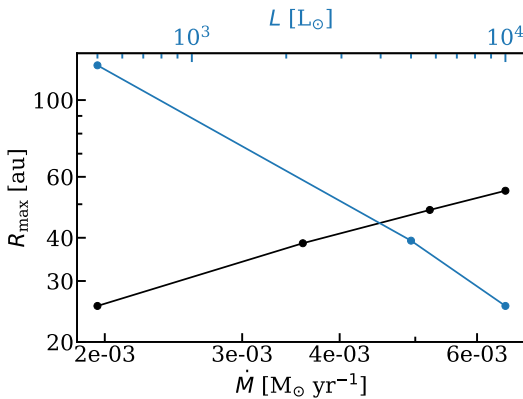
Figure 8.6: Maximum radius at which the midplane temperature is higher than the surface temperature as a function of mass accretion rate (black) and luminosity (blue). The models shown here are fiducial envelope-plus-disk models with large grains (i.e., high mm opacity dust), where M_E ( \dot{M} ) changes for the black line and L changes for the blue line.
