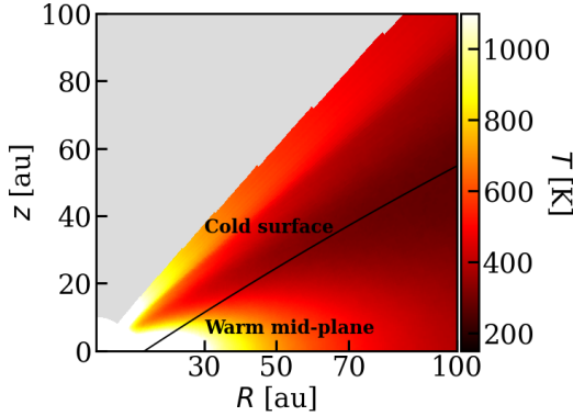
Figure 8.5: Two-dimensional map of the temperature for the fiducial envelope-plus-disk model, but with the difference that this model has high mm opacity dust and an envelope mass of 800 M_{\odot} ( \dot{M} = 5.2 \times 10^{-3} M_{\odot} \text{ yr}^{-1} ). The black contour shows the approximate location of the disk. In the inner disk ( R \lesssim 50 - 60 \text{ au} ), the midplane temperature is higher than the disk surface and envelope temperature.
