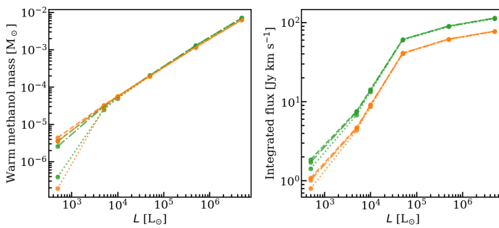
Figure 8.B.10: Same as Fig. 8.13, but dashed lines show the carved region with a size of 50 au, dash-dotted lines show the same for 200 au, and the dotted lines show the same for 500 au.
